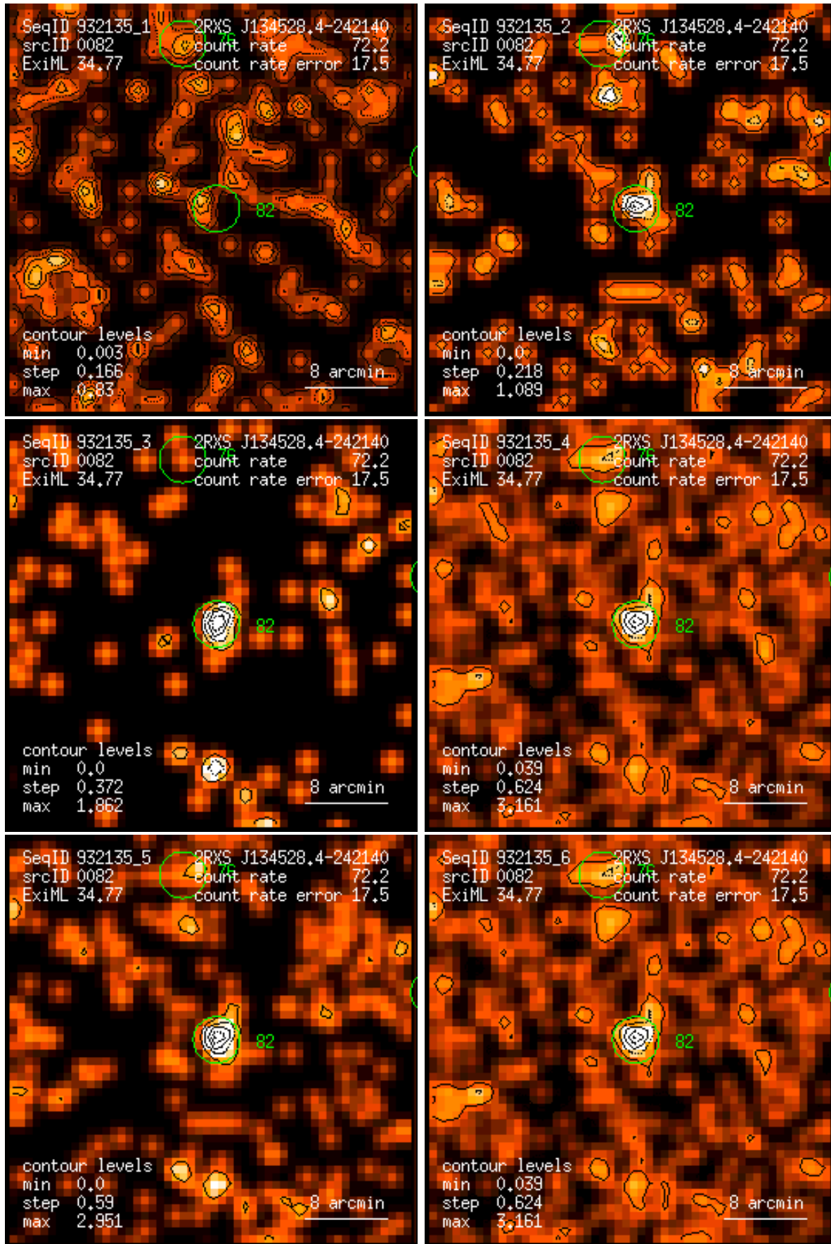
Figure 82: RASS 932135: detection 0082: band rate images, Gaussian filter: (1) PSPC channels 11 – 41, (2) 52 – 90, (3) 91 – 201, (4) 11 – 235, (5) 52 – 201, (6) 11 – 201. Broad band rates in counts/ks. Band rate contour levels in counts/ks/arcmin 2 .
