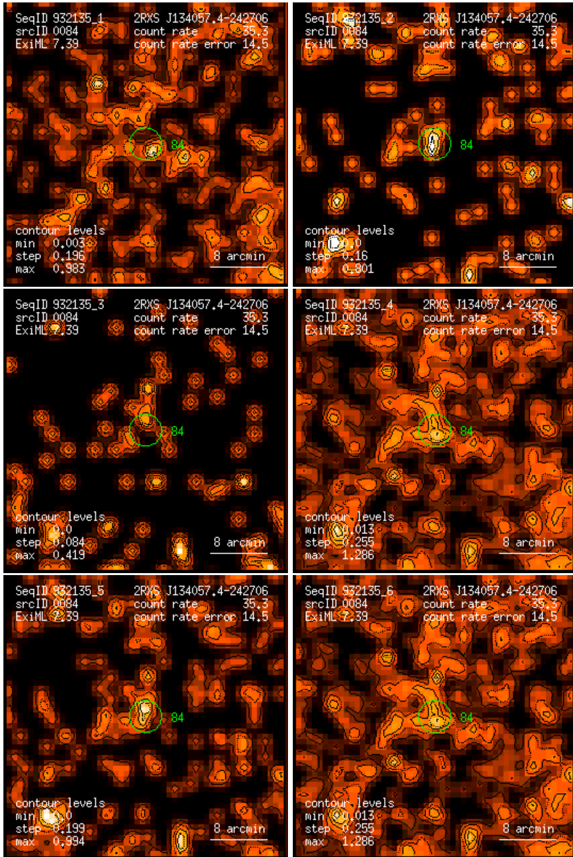
Figure 84: RASS 932135: detection 0084: band rate images, Gaussian filter: (1) PSPC channels 11 – 41, (2) 52 – 90, (3) 91 – 201, (4) 11 – 235, (5) 52 – 201, (6) 11 – 201. Broad band rates in counts/ks. Band rate contour levels in counts/ks/arcmin 2 .
