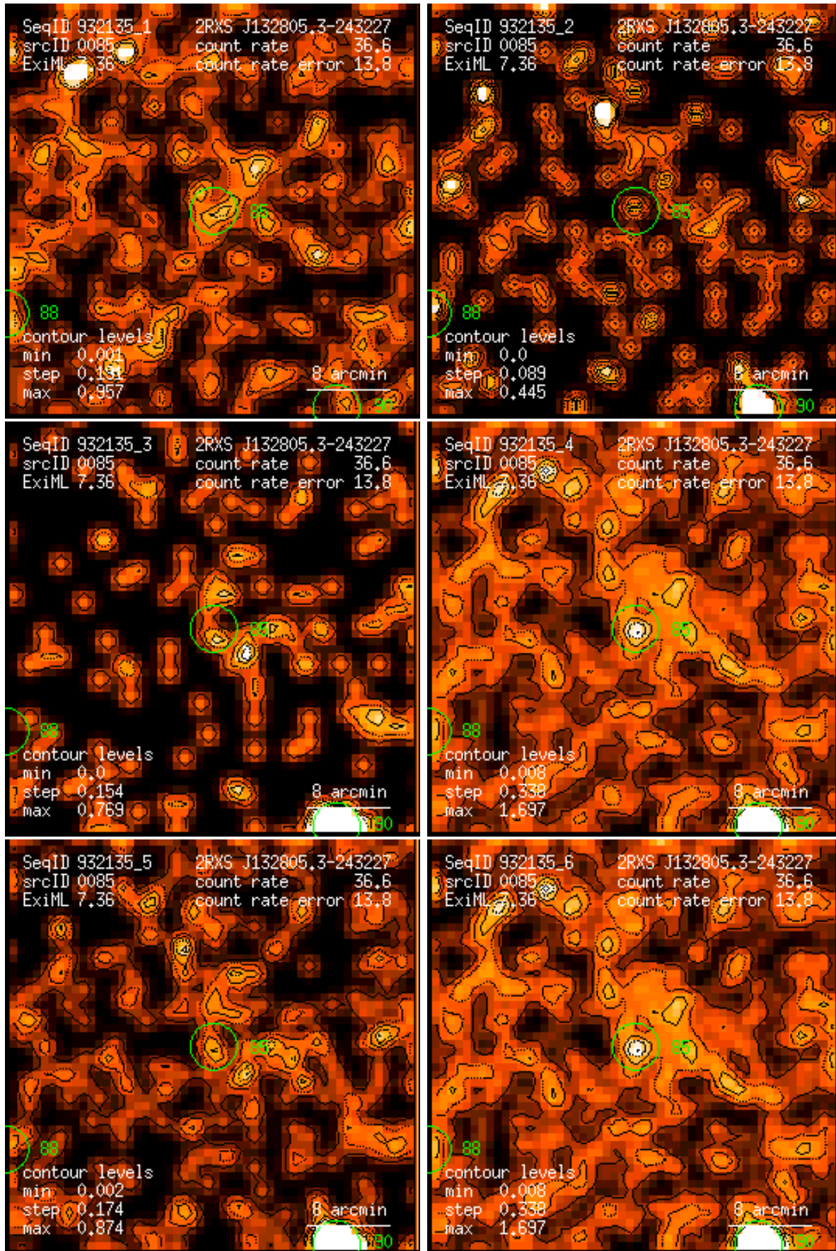
Figure 85: RASS 932135: detection 0085: band rate images, Gaussian filter: (1) PSPC channels 11 – 41, (2) 52 – 90, (3) 91 – 201, (4) 11 – 235, (5) 52 – 201, (6) 11 – 201. Broad band rates in counts/ks. Band rate contour levels in counts/ks/arcmin 2 .
