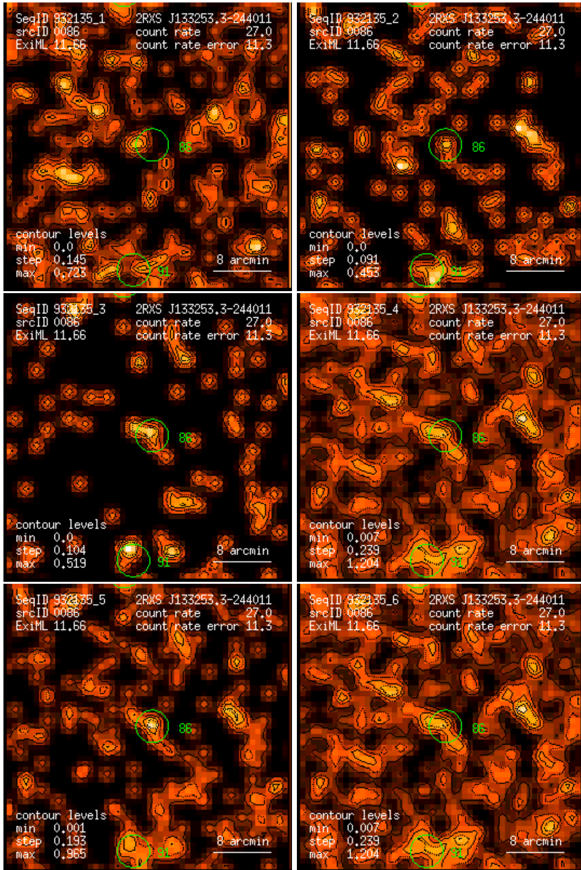
Figure 86: RASS 932135: detection 0086: band rate images, Gaussian filter: (1) PSPC channels 11 – 41, (2) 52 – 90, (3) 91 – 201, (4) 11 – 235, (5) 52 – 201, (6) 11 – 201. Broad band rates in counts/ks. Band rate contour levels in counts/ks/arcmin 2 .
