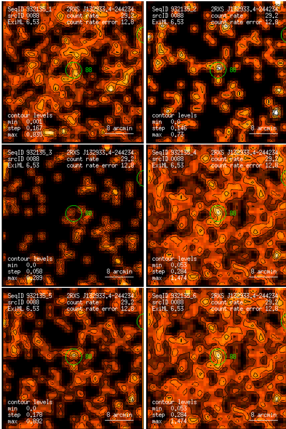
Figure 88: RASS 932135: detection 0088: band rate images, Gaussian filter: (1) PSPC channels 11 – 41, (2) 52 – 90, (3) 91 – 201, (4) 11 – 235, (5) 52 – 201, (6) 11 – 201. Broad band rates in counts/ks. Band rate contour levels in counts/ks/arcmin 2 .
