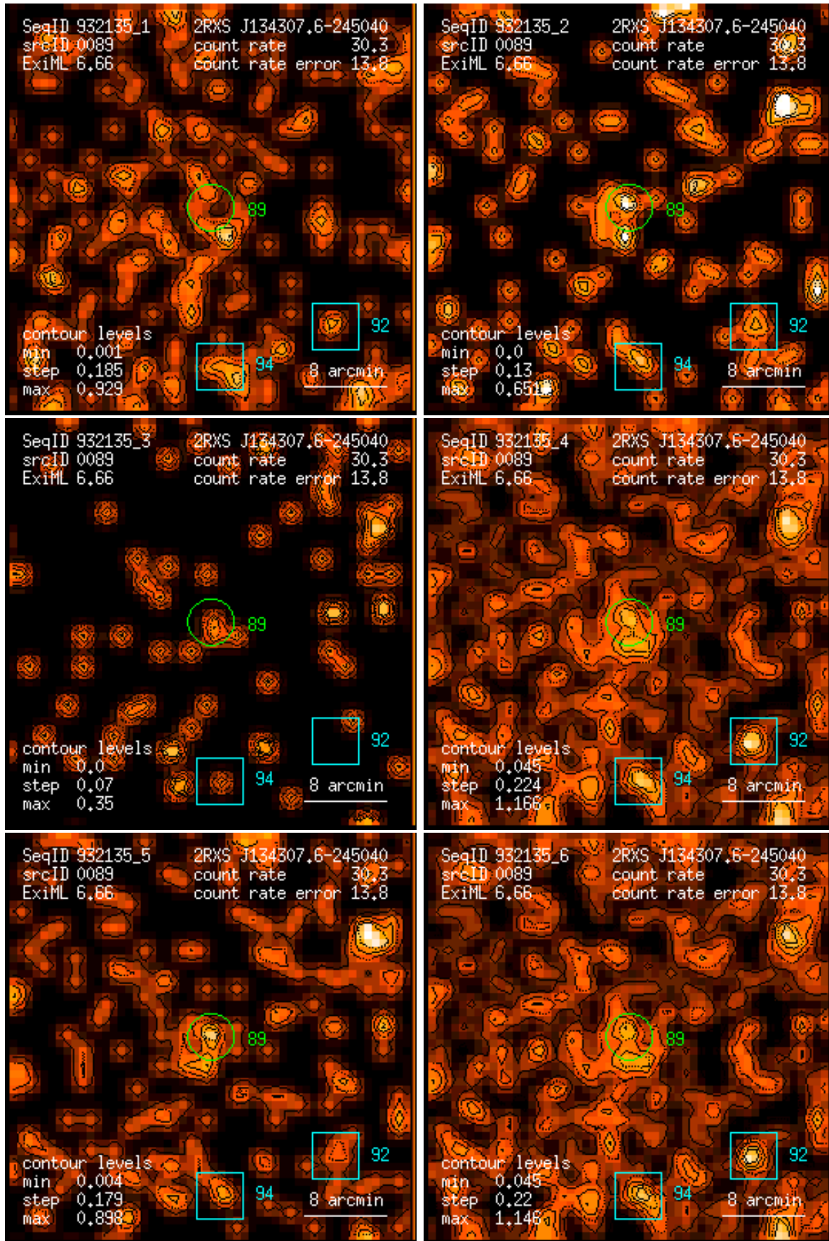
Figure 89: RASS 932135: detection 0089: band rate images, Gaussian filter: (1) PSPC channels 11 – 41, (2) 52 – 90, (3) 91 – 201, (4) 11 – 235, (5) 52 – 201, (6) 11 – 201. Broad band rates in counts/ks. Band rate contour levels in counts/ks/arcmin 2 .
