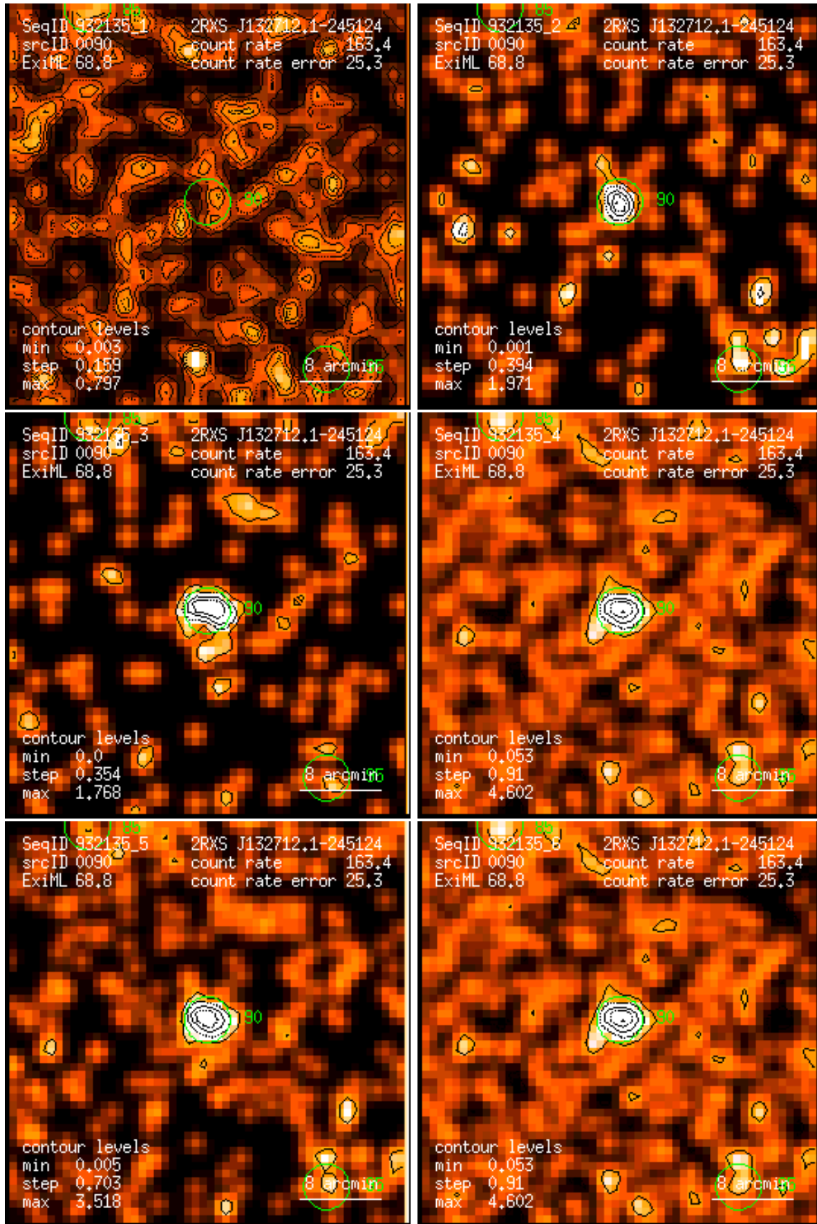
Figure 90: RASS 932135: detection 0090: band rate images, Gaussian filter: (1) PSPC channels 11 – 41, (2) 52 – 90, (3) 91 – 201, (4) 11 – 235, (5) 52 – 201, (6) 11 – 201. Broad band rates in counts/ks. Band rate contour levels in counts/ks/arcmin 2 .
