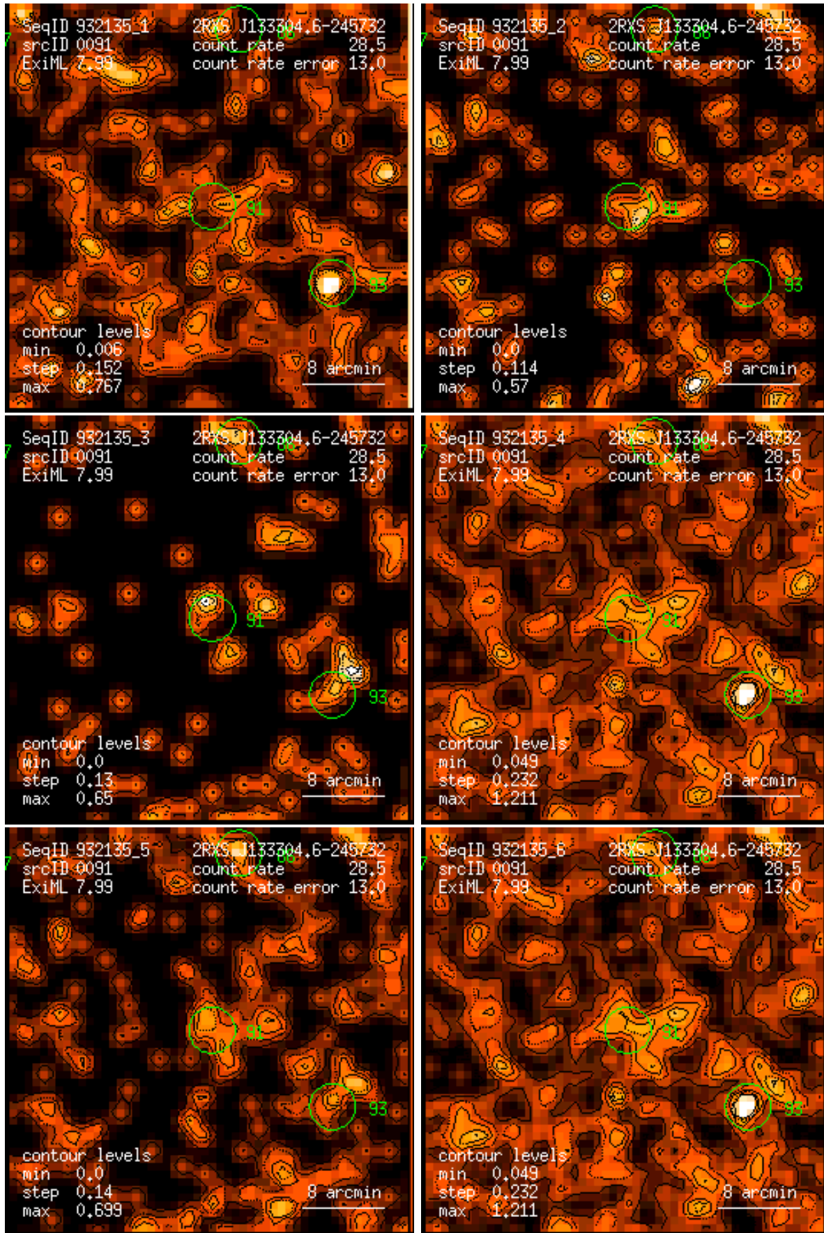
Figure 91: RASS 932135: detection 0091: band rate images, Gaussian filter: (1) PSPC channels 11 – 41, (2) 52 – 90, (3) 91 – 201, (4) 11 – 235, (5) 52 – 201, (6) 11 – 201. Broad band rates in counts/ks. Band rate contour levels in counts/ks/arcmin 2 .
