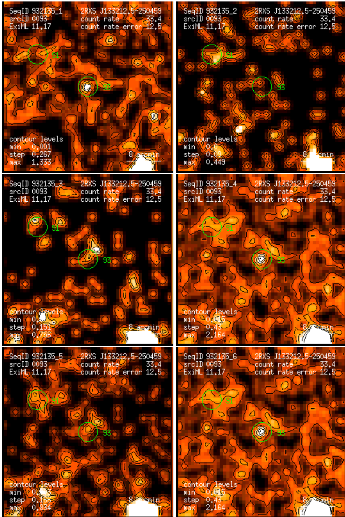
Figure 93: RASS 932135: detection 0093: band rate images, Gaussian filter: (1) PSPC channels 11 – 41, (2) 52 – 90, (3) 91 – 201, (4) 11 – 235, (5) 52 – 201, (6) 11 – 201. Broad band rates in counts/ks. Band rate contour levels in counts/ks/arcmin 2 .
