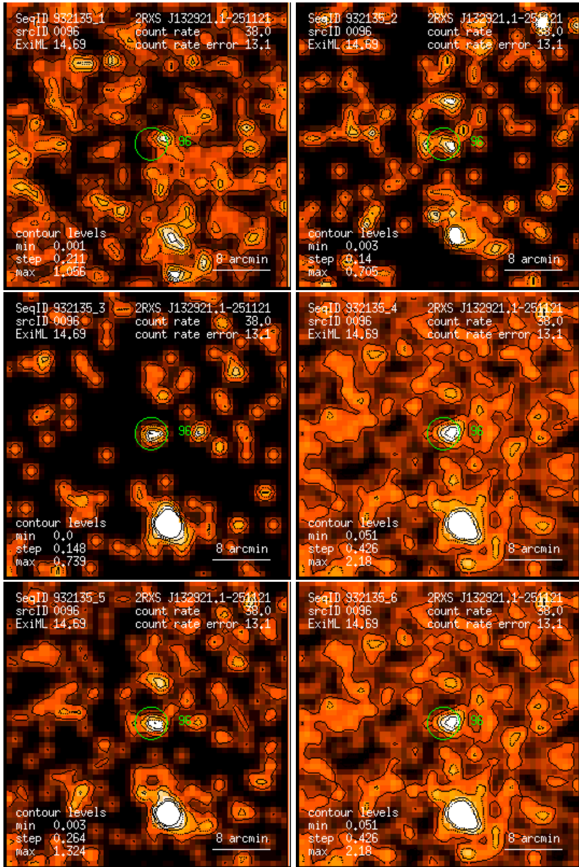
Figure 96: RASS 932135: detection 0096: band rate images, Gaussian filter: (1) PSPC channels 11 – 41, (2) 52 – 90, (3) 91 – 201, (4) 11 – 235, (5) 52 – 201, (6) 11 – 201. Broad band rates in counts/ks. Band rate contour levels in counts/ks/arcmin 2 .
