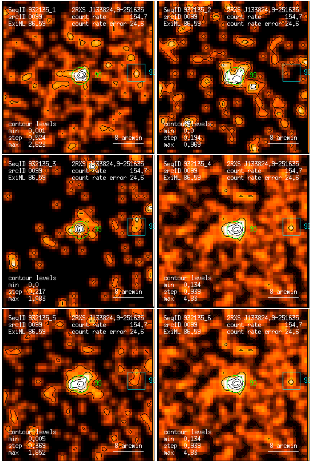
Figure 99: RASS 932135: detection 0099: band rate images, Gaussian filter: (1) PSPC channels 11 – 41, (2) 52 – 90, (3) 91 – 201, (4) 11 – 235, (5) 52 – 201, (6) 11 – 201. Broad band rates in counts/ks. Band rate contour levels in counts/ks/arcmin 2 .
