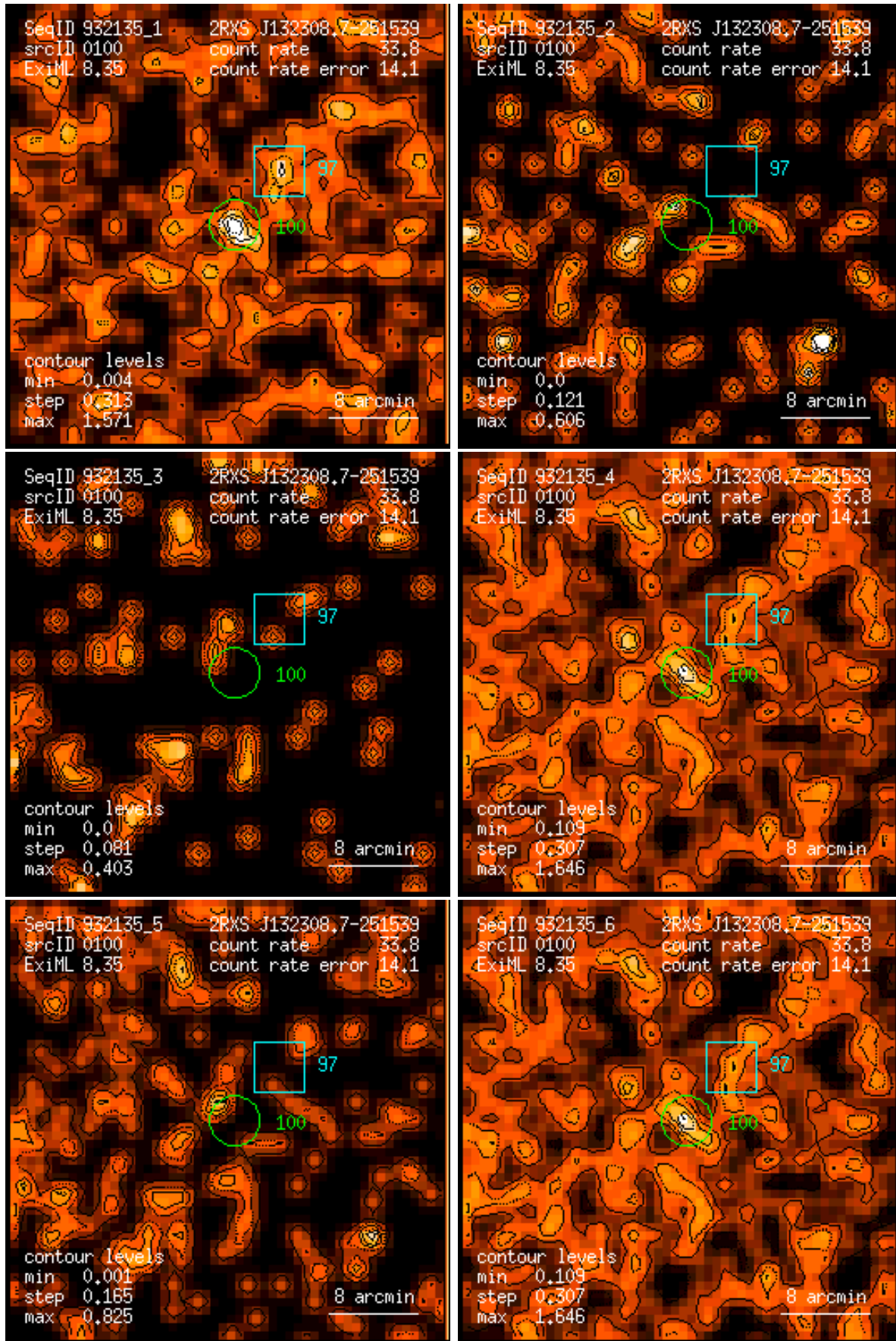
Figure 100: RASS 932135: detection 0100: band rate images, Gaussian filter: (1) PSPC channels 11 – 41, (2) 52 – 90, (3) 91 – 201, (4) 11 – 235, (5) 52 – 201, (6) 11 – 201. Broad band rates in counts/ks. Band rate contour levels in counts/ks/arcmin 2 .
