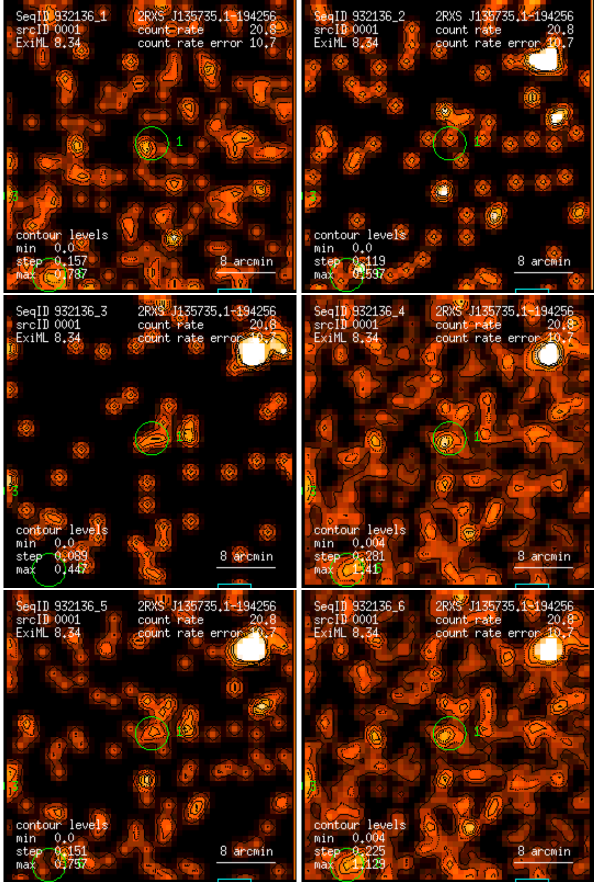
Figure 1: RASS 932136: detection 0001: band rate images, Gaussian filter: (1) PSPC channels 11 – 41, (2) 52 – 90, (3) 91 – 201, (4) 11 – 235, (5) 52 – 201, (6) 11 – 201. Broad band rates in counts/ks. Band rate contour levels in counts/ks/arcmin 2 .
