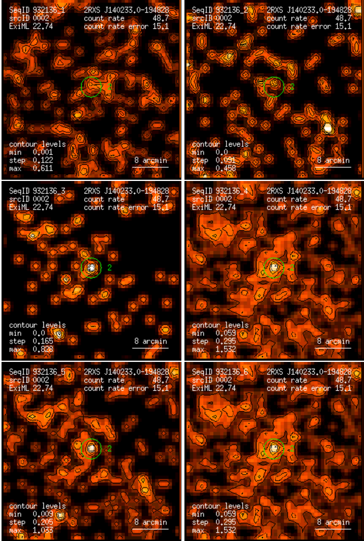
Figure 2: RASS 932136: detection 0002: band rate images, Gaussian filter: (1) PSPC channels 11 – 41, (2) 52 – 90, (3) 91 – 201, (4) 11 – 235, (5) 52 – 201, (6) 11 – 201. Broad band rates in counts/ks. Band rate contour levels in counts/ks/arcmin 2 .
