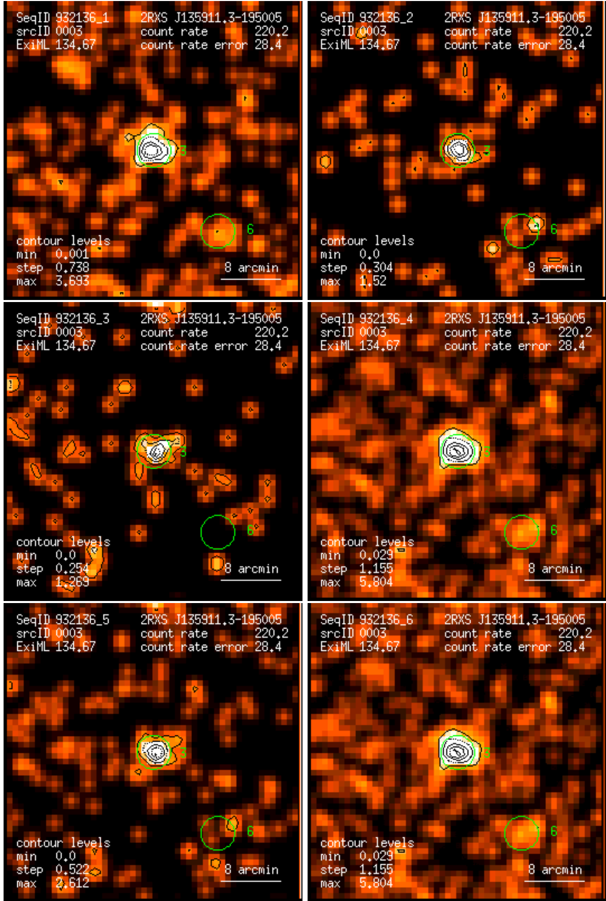
Figure 3: RASS 932136: detection 0003: band rate images, Gaussian filter: (1) PSPC channels 11 – 41, (2) 52 – 90, (3) 91 – 201, (4) 11 – 235, (5) 52 – 201, (6) 11 – 201. Broad band rates in counts/ks. Band rate contour levels in counts/ks/arcmin 2 .
