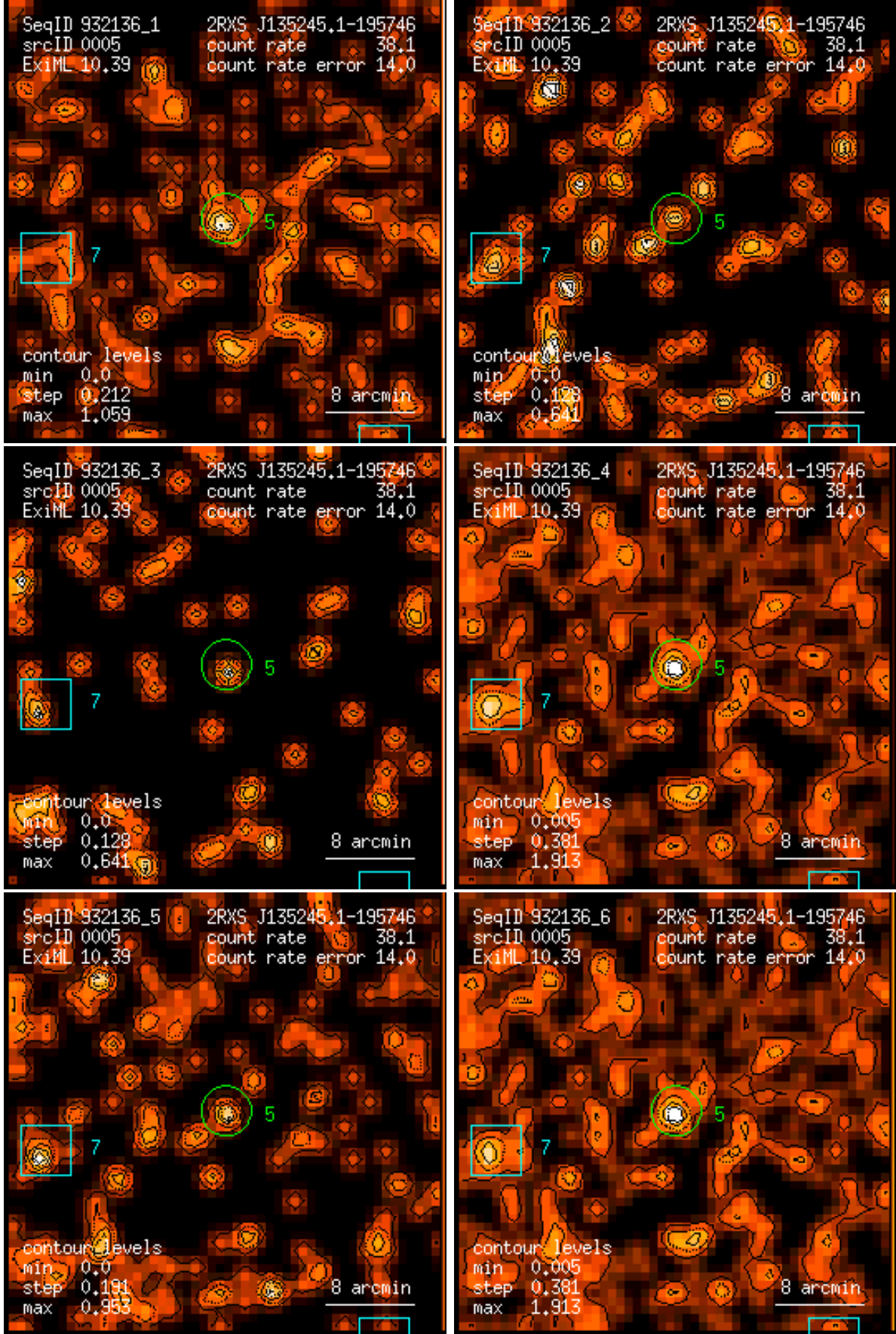
Figure 5: RASS 932136: detection 0005: band rate images, Gaussian filter: (1) PSPC channels 11 – 41, (2) 52 – 90, (3) 91 – 201, (4) 11 – 235, (5) 52 – 201, (6) 11 – 201. Broad band rates in counts/ks. Band rate contour levels in counts/ks/arcmin 2 .
