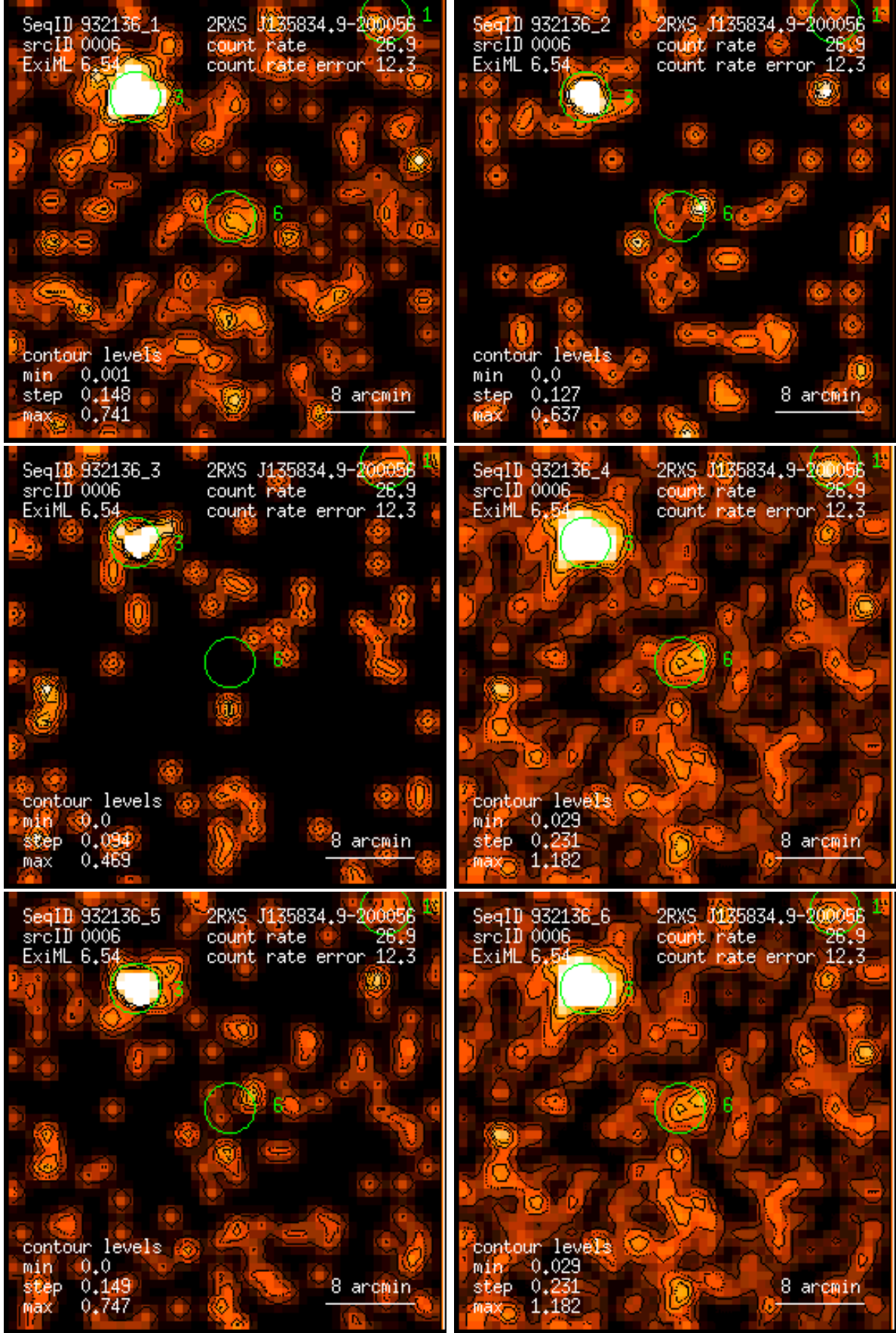
Figure 6: RASS 932136: detection 0006: band rate images, Gaussian filter: (1) PSPC channels 11 – 41, (2) 52 – 90, (3) 91 – 201, (4) 11 – 235, (5) 52 – 201, (6) 11 – 201. Broad band rates in counts/ks. Band rate contour levels in counts/ks/arcmin 2 .
