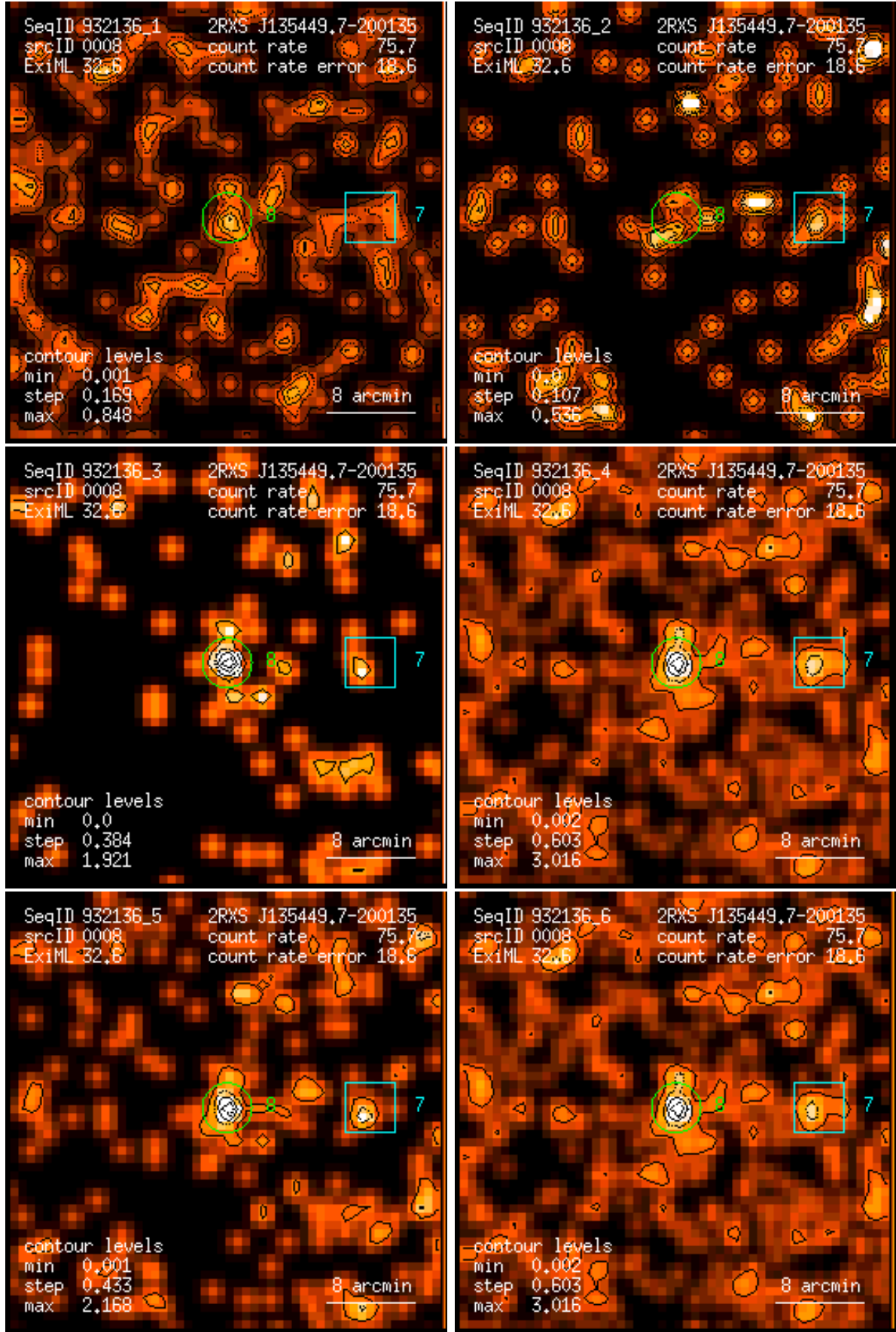
Figure 8: RASS 932136: detection 0008: band rate images, Gaussian filter: (1) PSPC channels 11 – 41, (2) 52 – 90, (3) 91 – 201, (4) 11 – 235, (5) 52 – 201, (6) 11 – 201. Broad band rates in counts/ks. Band rate contour levels in counts/ks/arcmin 2 .
