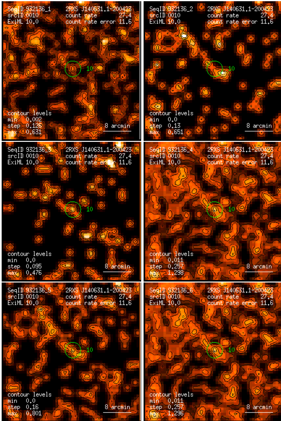
Figure 10: RASS 932136: detection 0010: band rate images, Gaussian filter: (1) PSPC channels 11 – 41, (2) 52 – 90, (3) 91 – 201, (4) 11 – 235, (5) 52 – 201, (6) 11 – 201. Broad band rates in counts/ks. Band rate contour levels in counts/ks/arcmin 2 .
