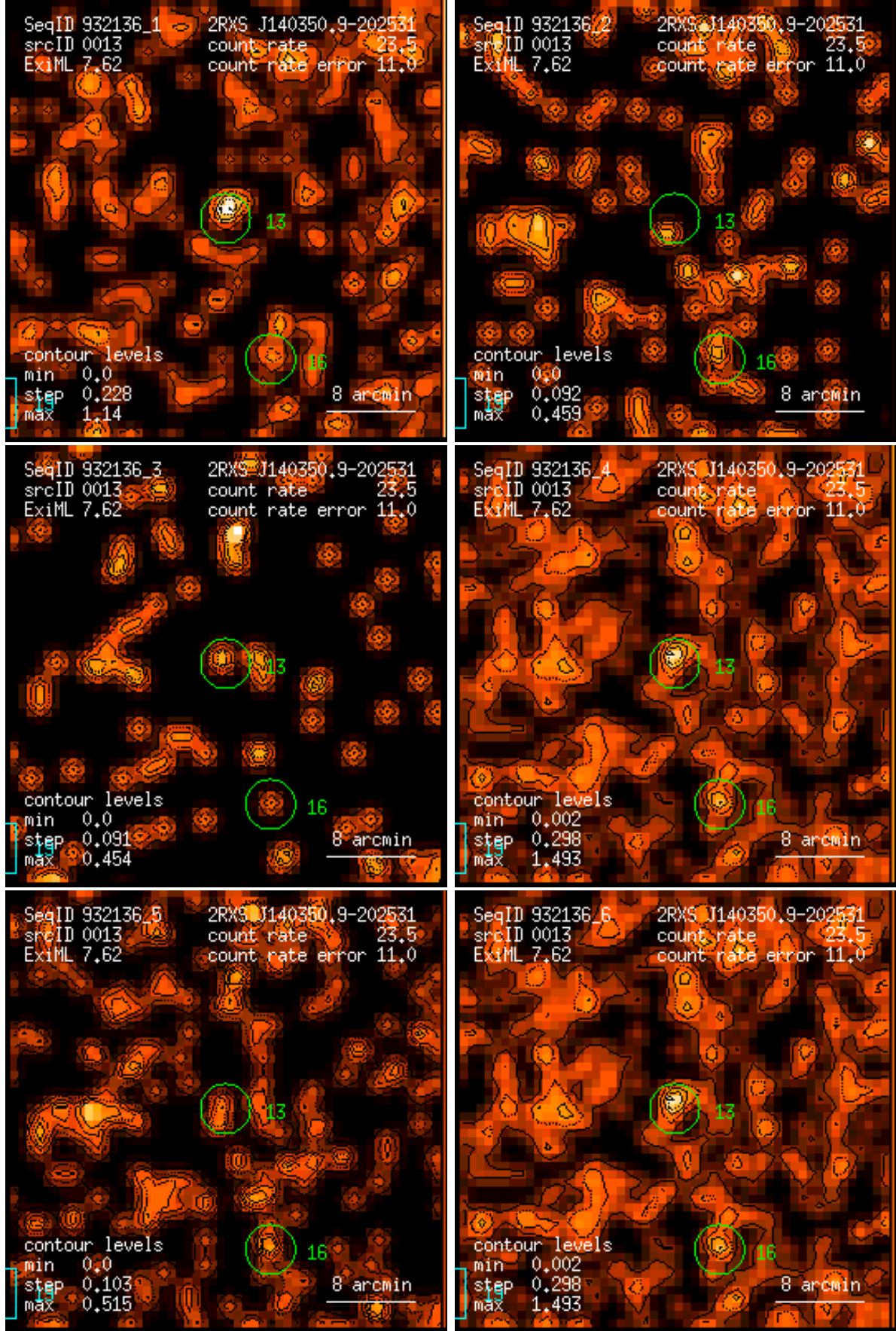
Figure 13: RASS 932136: detection 0013: band rate images, Gaussian filter: (1) PSPC channels 11 – 41, (2) 52 – 90, (3) 91 – 201, (4) 11 – 235, (5) 52 – 201, (6) 11 – 201. Broad band rates in counts/ks. Band rate contour levels in counts/ks/arcmin 2 .
