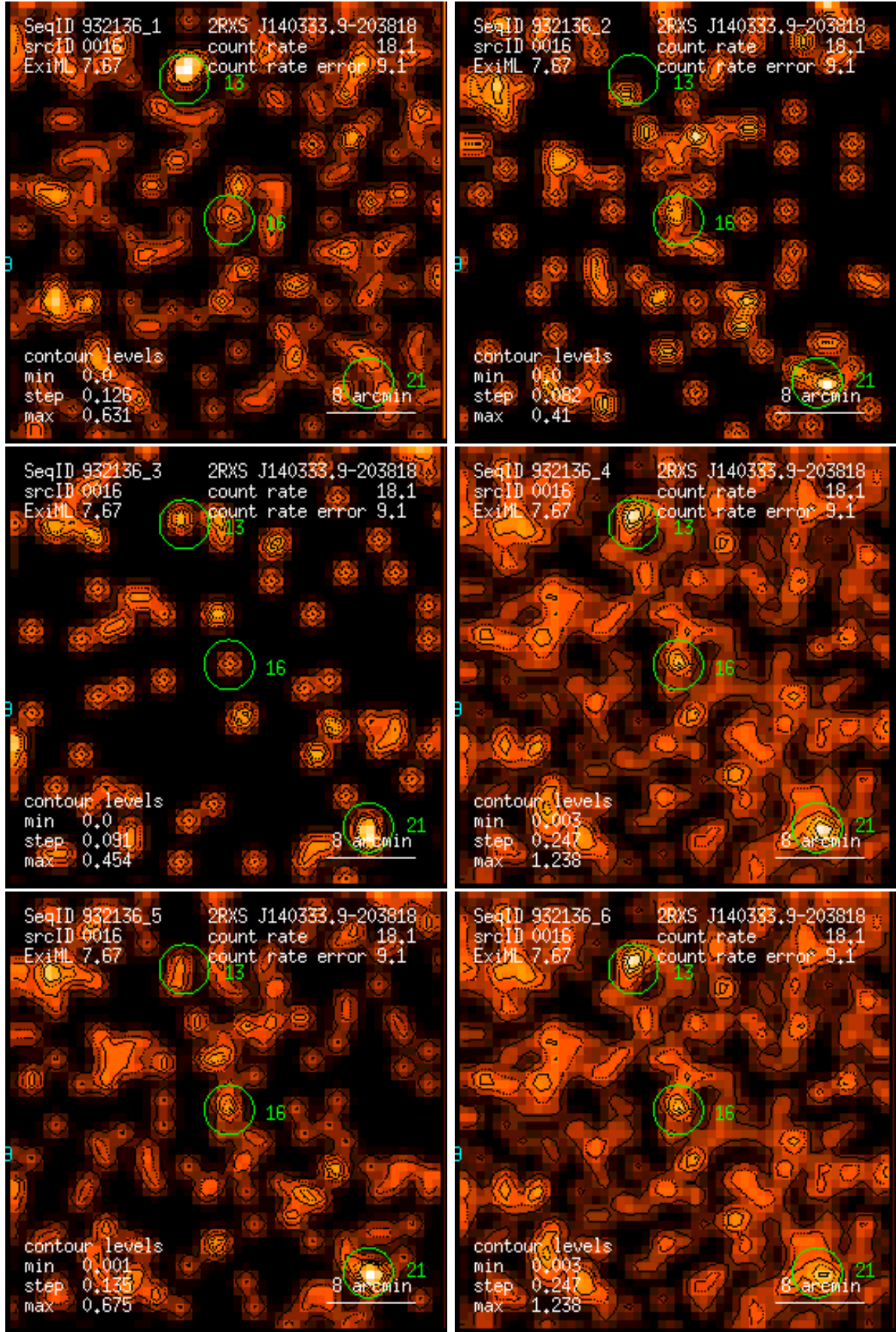
Figure 16: RASS 932136: detection 0016: band rate images, Gaussian filter: (1) PSPC channels 11 – 41, (2) 52 – 90, (3) 91 – 201, (4) 11 – 235, (5) 52 – 201, (6) 11 – 201. Broad band rates in counts/ks. Band rate contour levels in counts/ks/arcmin 2 .
