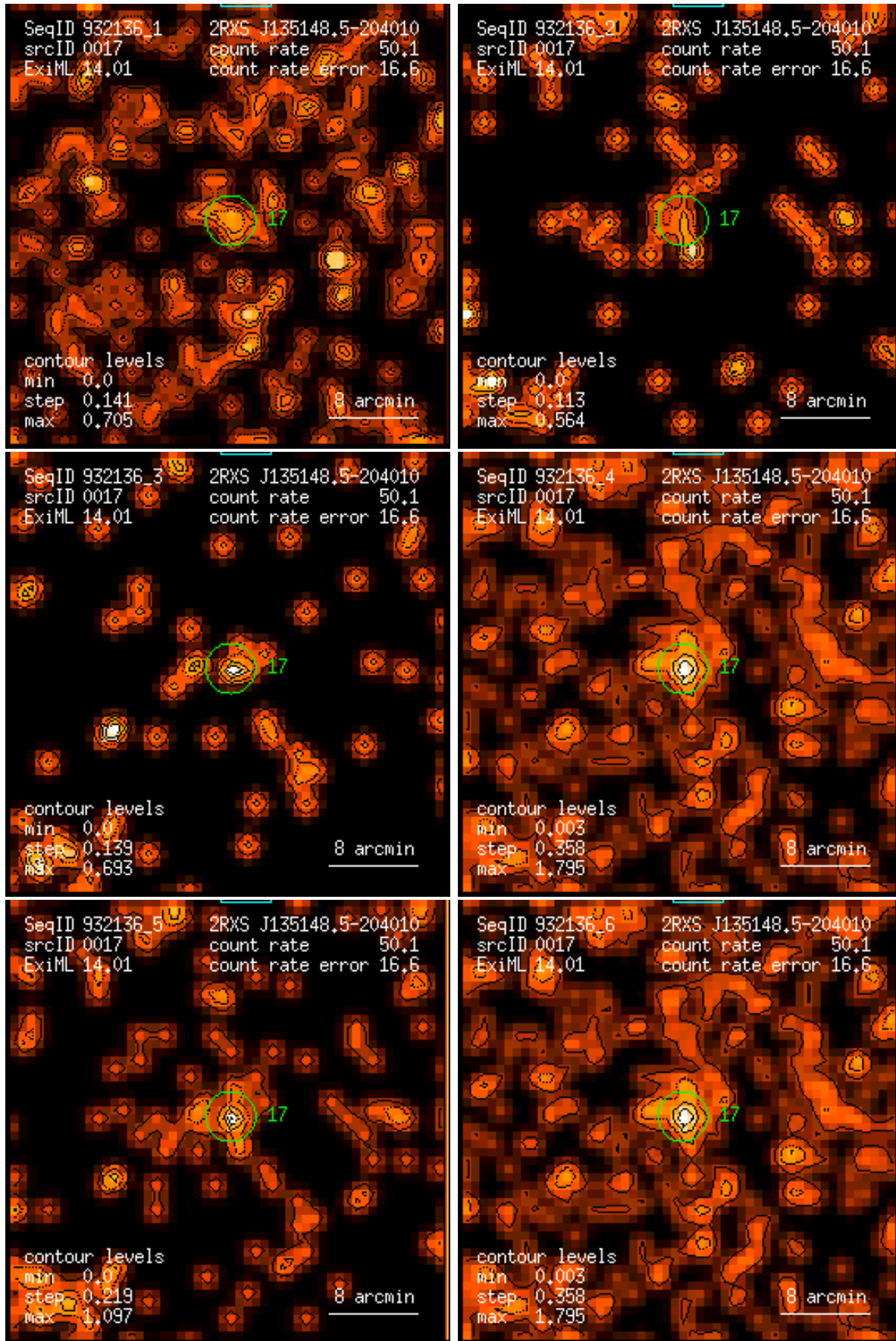
Figure 17: RASS 932136: detection 0017: band rate images, Gaussian filter: (1) PSPC channels 11 – 41, (2) 52 – 90, (3) 91 – 201, (4) 11 – 235, (5) 52 – 201, (6) 11 – 201. Broad band rates in counts/ks. Band rate contour levels in counts/ks/arcmin 2 .
