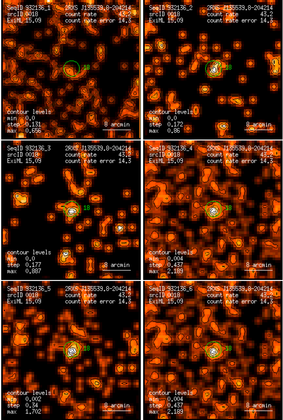
Figure 18: RASS 932136: detection 0018: band rate images, Gaussian filter: (1) PSPC channels 11 – 41, (2) 52 – 90, (3) 91 – 201, (4) 11 – 235, (5) 52 – 201, (6) 11 – 201. Broad band rates in counts/ks. Band rate contour levels in counts/ks/arcmin 2 .
