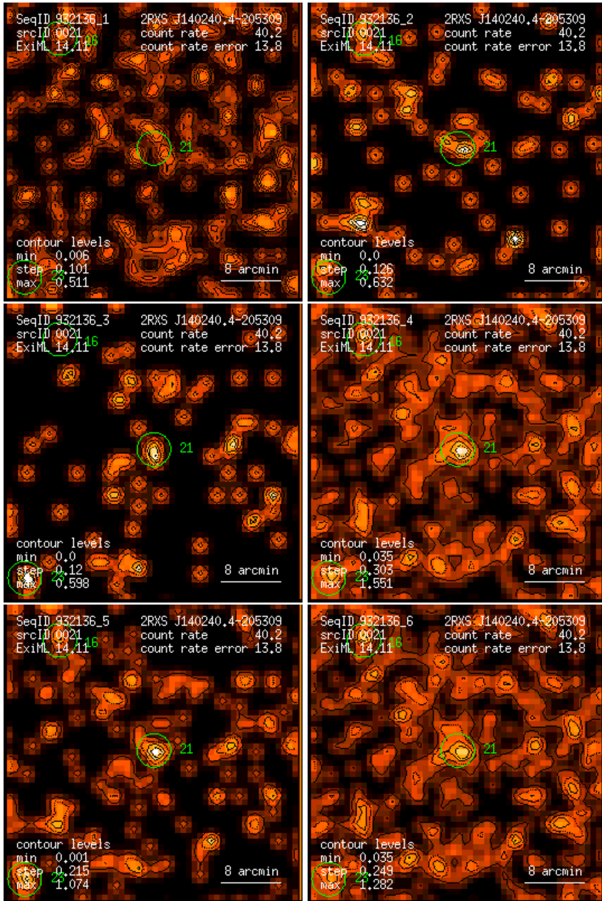
Figure 21: RASS 932136: detection 0021: band rate images, Gaussian filter: (1) PSPC channels 11 – 41, (2) 52 – 90, (3) 91 – 201, (4) 11 – 235, (5) 52 – 201, (6) 11 – 201. Broad band rates in counts/ks. Band rate contour levels in counts/ks/arcmin 2 .
