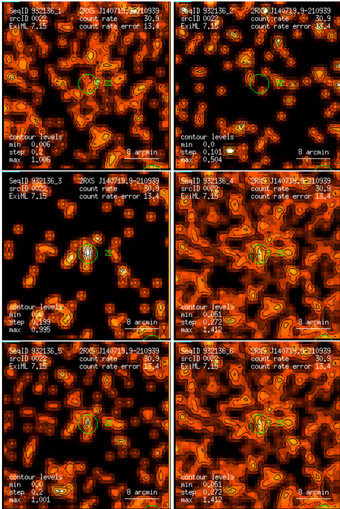
Figure 22: RASS 932136: detection 0022: band rate images, Gaussian filter: (1) PSPC channels 11 – 41, (2) 52 – 90, (3) 91 – 201, (4) 11 – 235, (5) 52 – 201, (6) 11 – 201. Broad band rates in counts/ks. Band rate contour levels in counts/ks/arcmin 2 .
