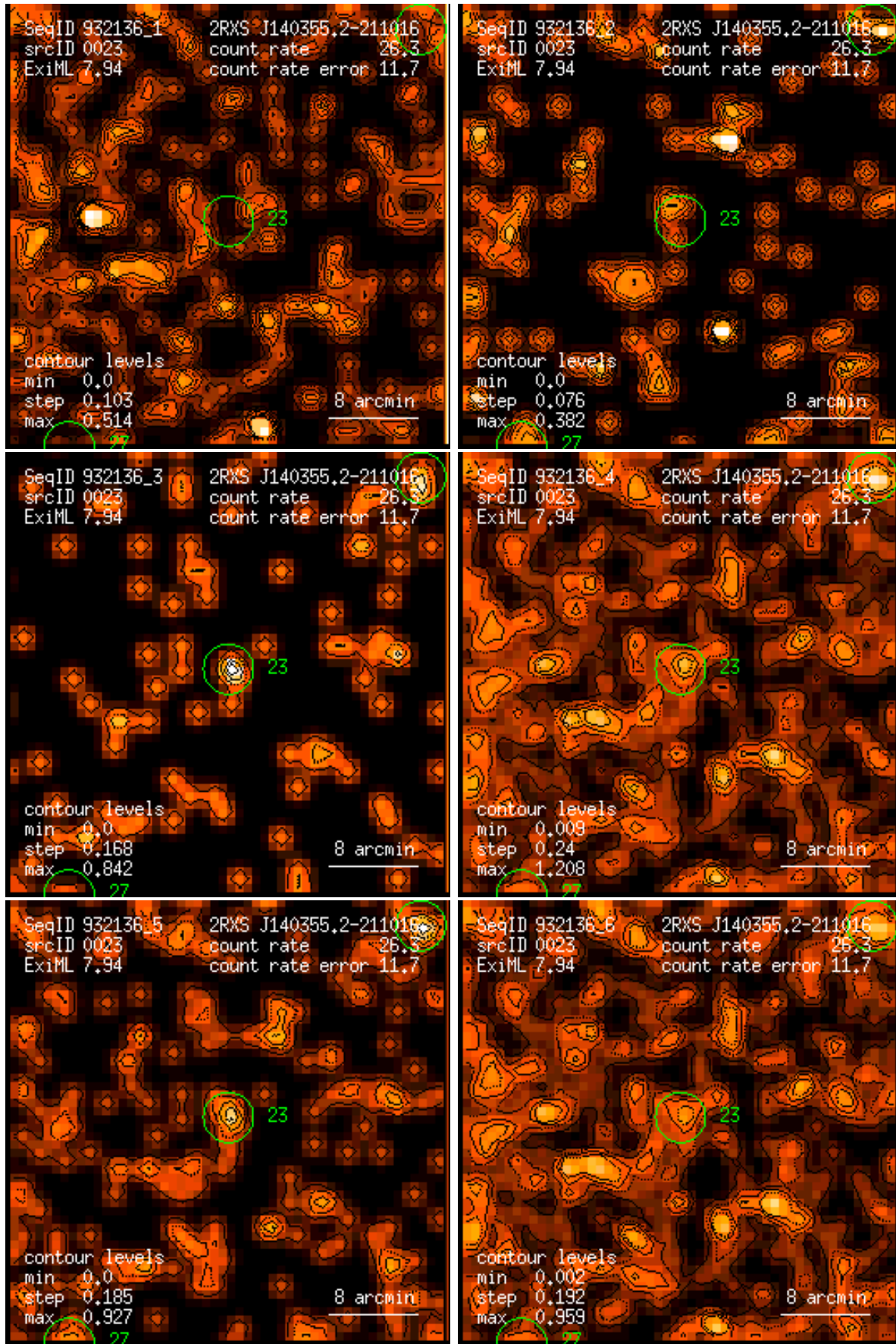
Figure 23: RASS 932136: detection 0023: band rate images, Gaussian filter: (1) PSPC channels 11 – 41, (2) 52 – 90, (3) 91 – 201, (4) 11 – 235, (5) 52 – 201, (6) 11 – 201. Broad band rates in counts/ks. Band rate contour levels in counts/ks/arcmin 2 .
