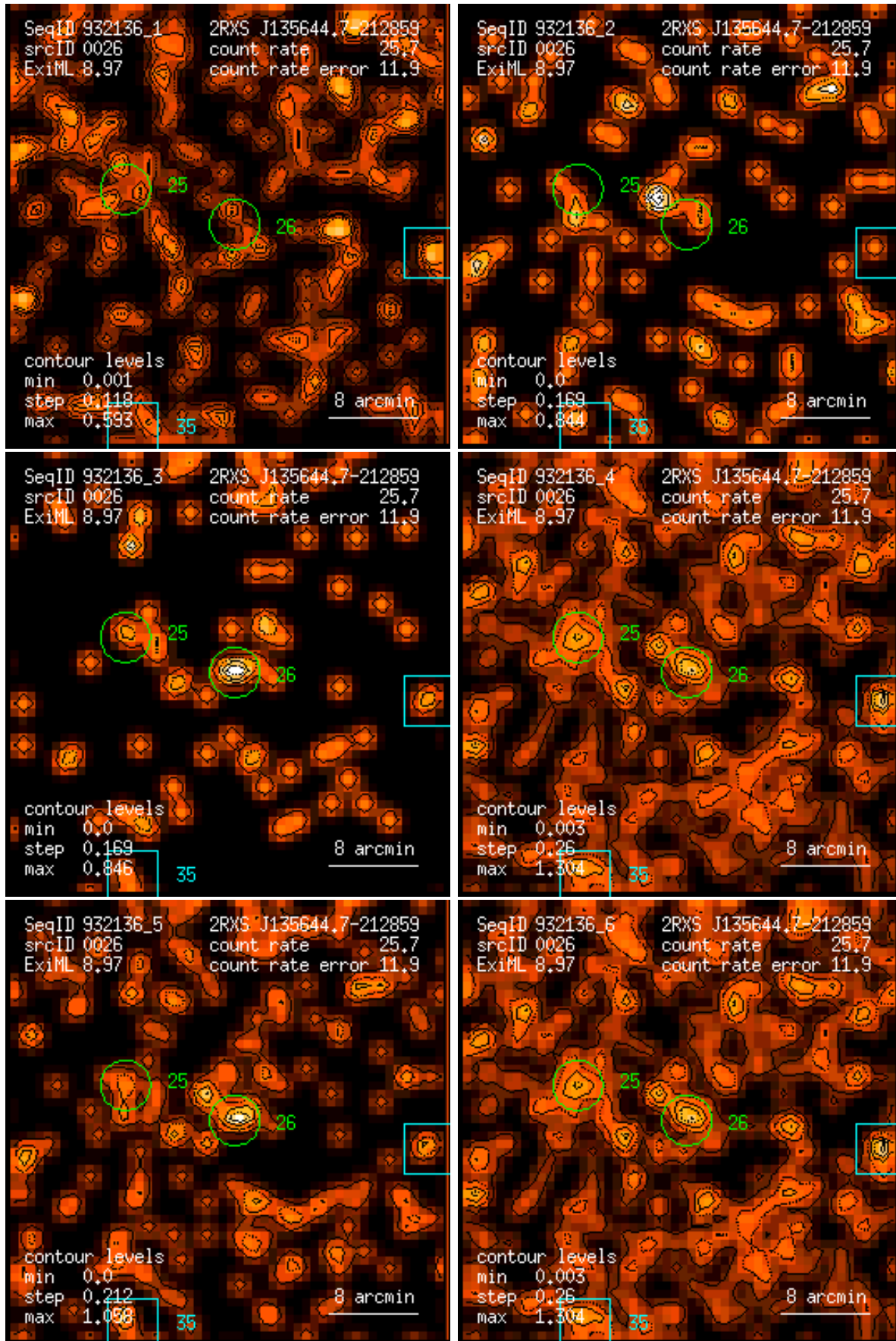
Figure 26: RASS 932136: detection 0026: band rate images, Gaussian filter: (1) PSPC channels 11 – 41, (2) 52 – 90, (3) 91 – 201, (4) 11 – 235, (5) 52 – 201, (6) 11 – 201. Broad band rates in counts/ks. Band rate contour levels in counts/ks/arcmin 2 .
