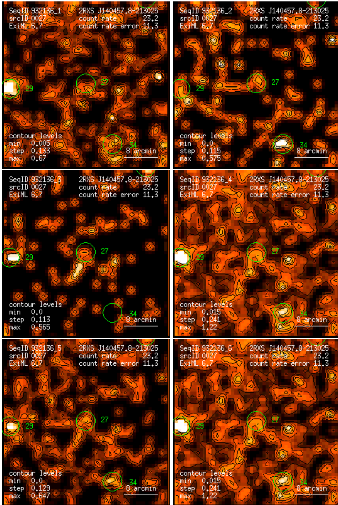
Figure 27: RASS 932136: detection 0027: band rate images, Gaussian filter: (1) PSPC channels 11 – 41, (2) 52 – 90, (3) 91 – 201, (4) 11 – 235, (5) 52 – 201, (6) 11 – 201. Broad band rates in counts/ks. Band rate contour levels in counts/ks/arcmin 2 .
