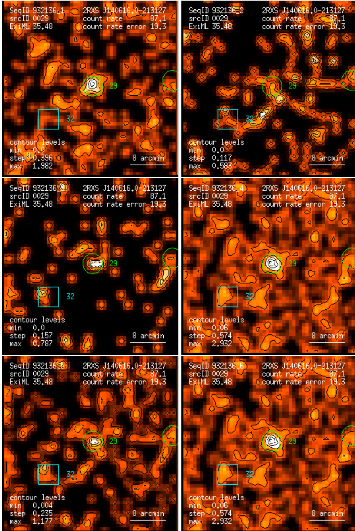
Figure 29: RASS 932136: detection 0029: band rate images, Gaussian filter: (1) PSPC channels 11 – 41, (2) 52 – 90, (3) 91 – 201, (4) 11 – 235, (5) 52 – 201, (6) 11 – 201. Broad band rates in counts/ks. Band rate contour levels in counts/ks/arcmin 2 .
