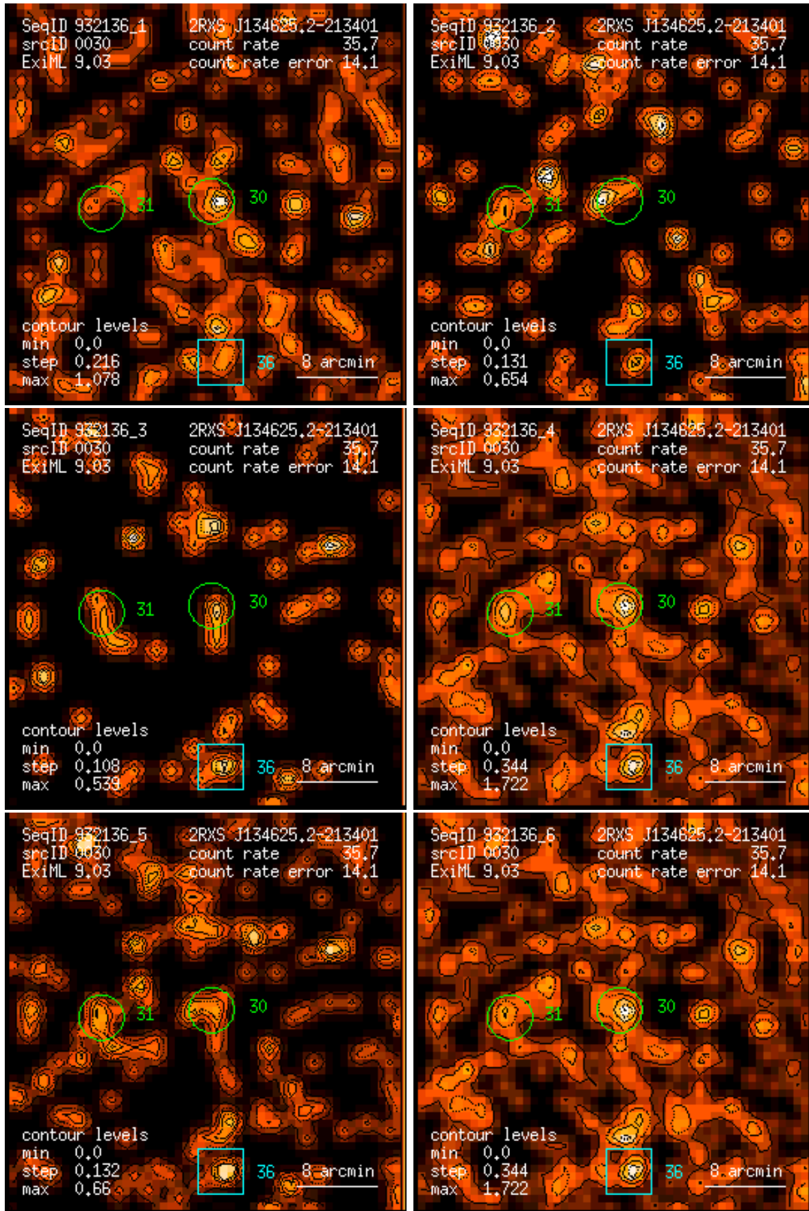
Figure 30: RASS 932136: detection 0030: band rate images, Gaussian filter: (1) PSPC channels 11 – 41, (2) 52 – 90, (3) 91 – 201, (4) 11 – 235, (5) 52 – 201, (6) 11 – 201. Broad band rates in counts/ks. Band rate contour levels in counts/ks/arcmin 2 .
