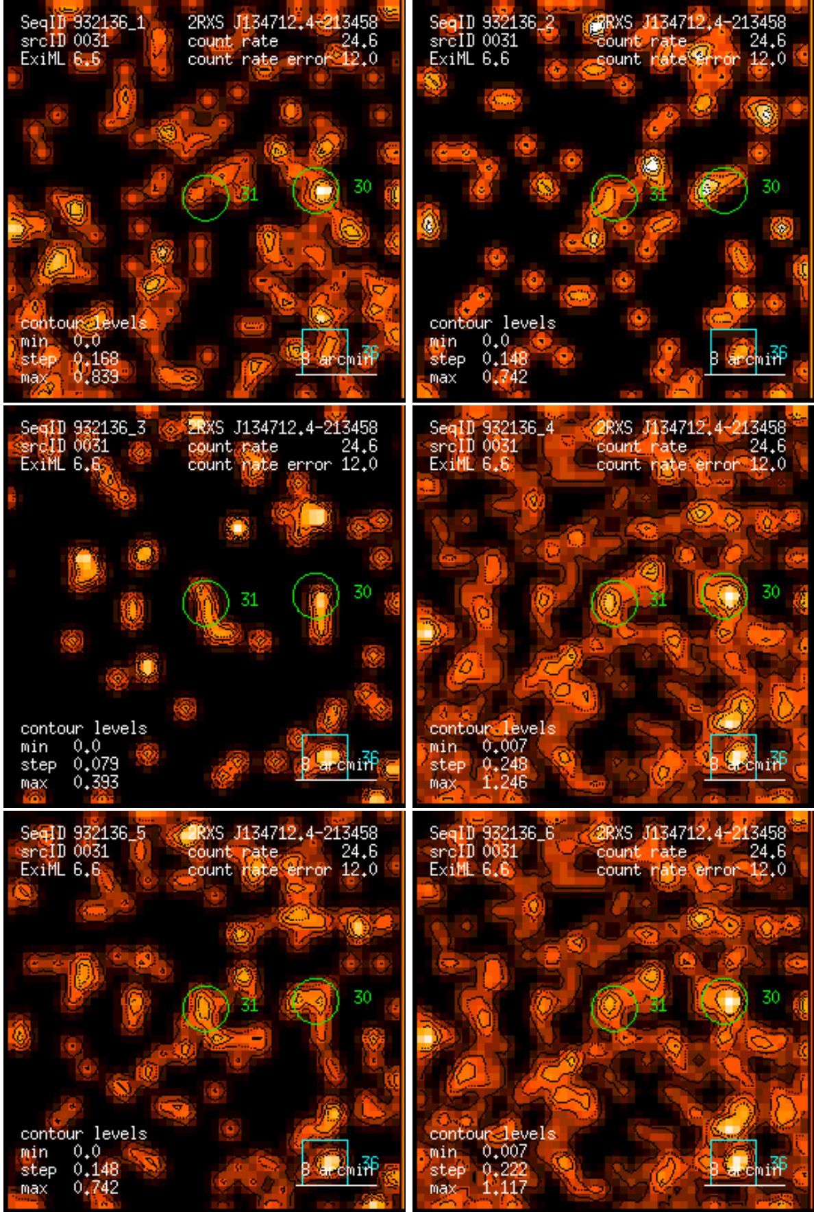
Figure 31: RASS 932136: detection 0031: band rate images, Gaussian filter: (1) PSPC channels 11 – 41, (2) 52 – 90, (3) 91 – 201, (4) 11 – 235, (5) 52 – 201, (6) 11 – 201. Broad band rates in counts/ks. Band rate contour levels in counts/ks/arcmin 2 .
