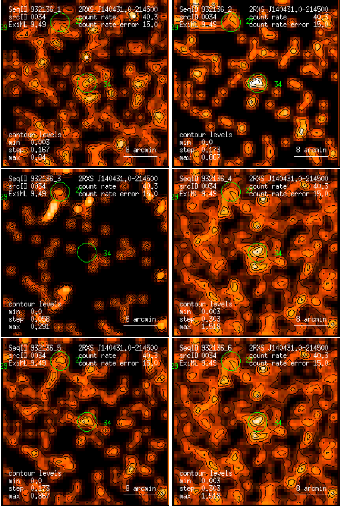
Figure 34: RASS 932136: detection 0034: band rate images, Gaussian filter: (1) PSPC channels 11 – 41, (2) 52 – 90, (3) 91 – 201, (4) 11 – 235, (5) 52 – 201, (6) 11 – 201. Broad band rates in counts/ks. Band rate contour levels in counts/ks/arcmin 2 .
