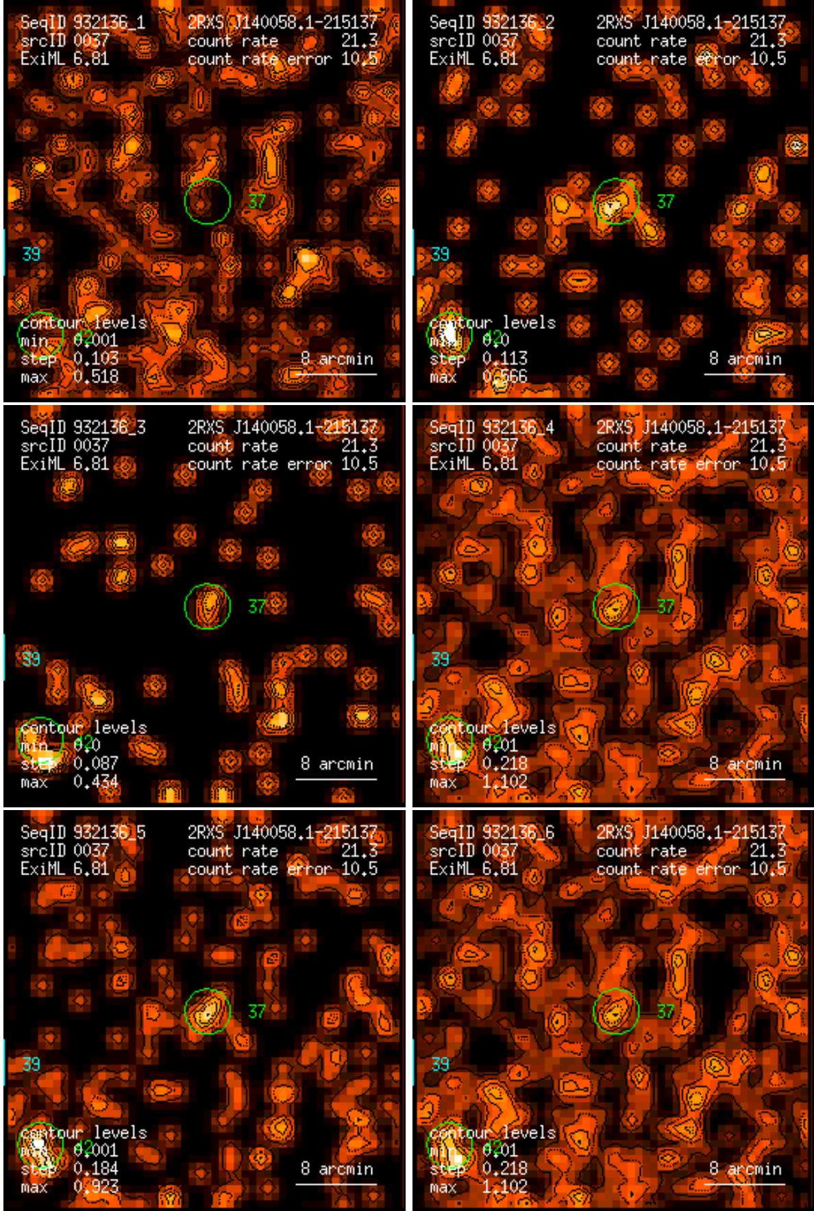
Figure 37: RASS 932136: detection 0037: band rate images, Gaussian filter: (1) PSPC channels 11 – 41, (2) 52 – 90, (3) 91 – 201, (4) 11 – 235, (5) 52 – 201, (6) 11 – 201. Broad band rates in counts/ks. Band rate contour levels in counts/ks/arcmin 2 .
