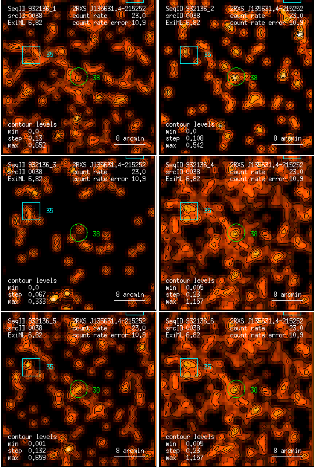
Figure 38: RASS 932136: detection 0038: band rate images, Gaussian filter: (1) PSPC channels 11 – 41, (2) 52 – 90, (3) 91 – 201, (4) 11 – 235, (5) 52 – 201, (6) 11 – 201. Broad band rates in counts/ks. Band rate contour levels in counts/ks/arcmin 2 .
