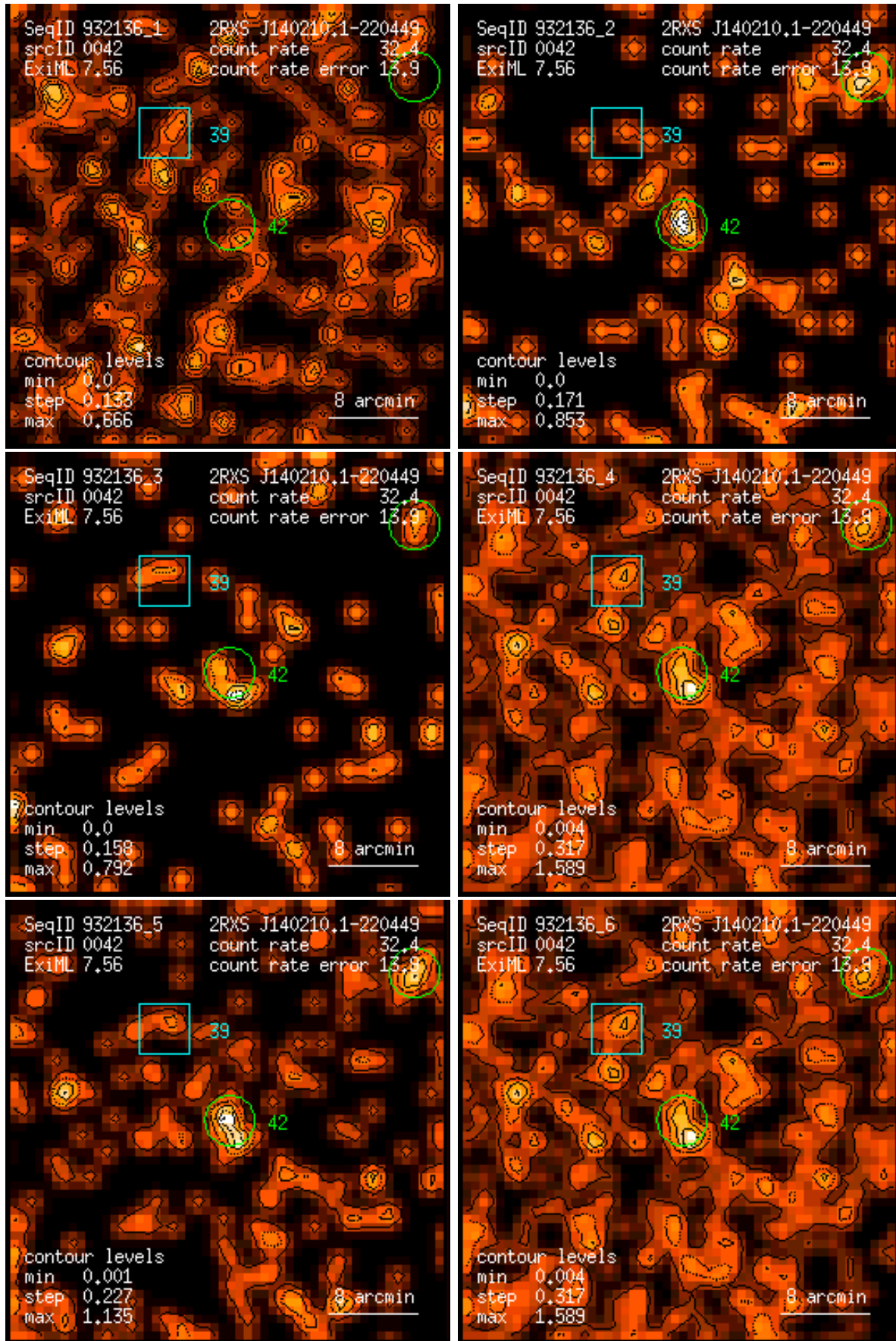
Figure 42: RASS 932136: detection 0042: band rate images, Gaussian filter: (1) PSPC channels 11 – 41, (2) 52 – 90, (3) 91 – 201, (4) 11 – 235, (5) 52 – 201, (6) 11 – 201. Broad band rates in counts/ks. Band rate contour levels in counts/ks/arcmin 2 .
