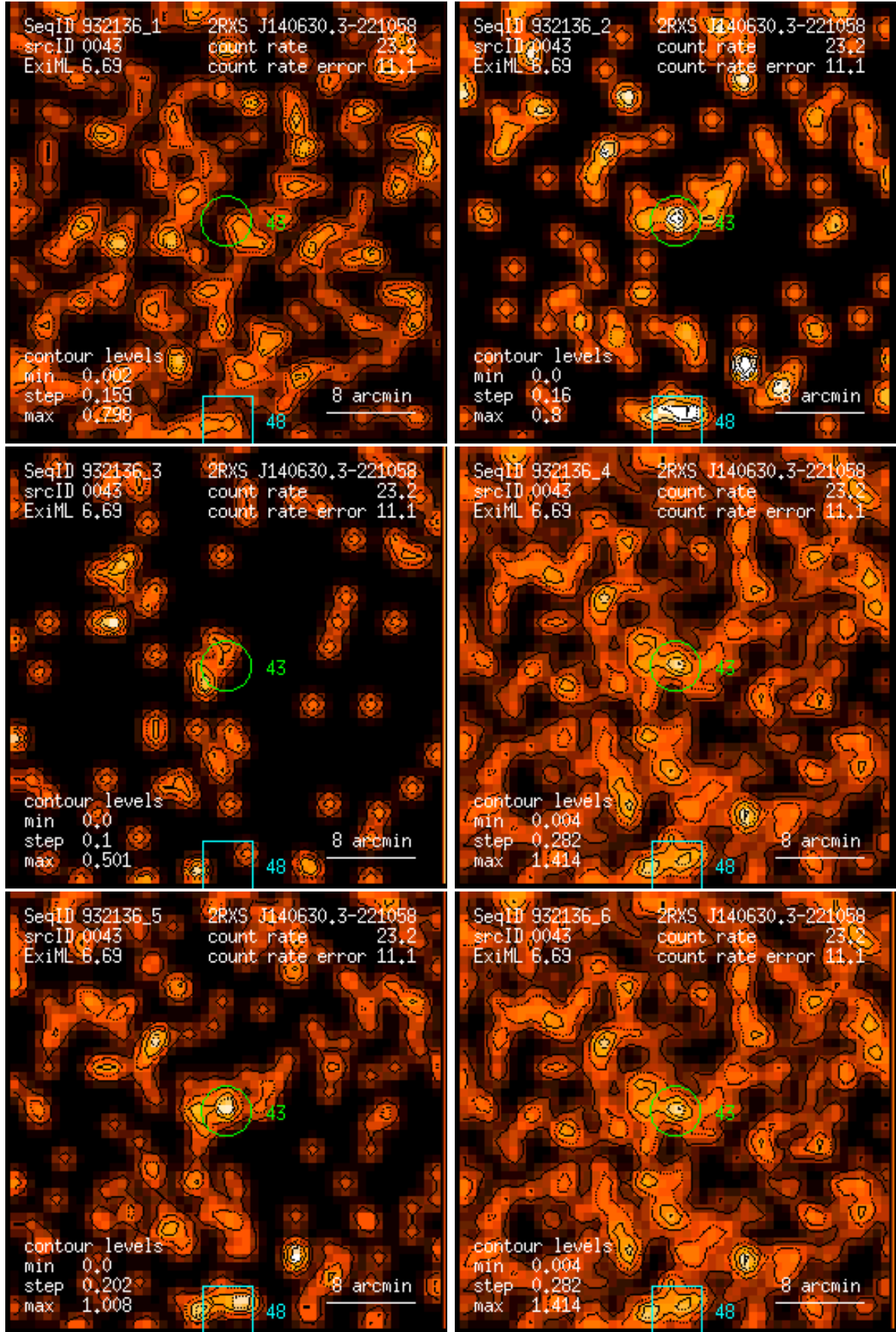
Figure 43: RASS 932136: detection 0043: band rate images, Gaussian filter: (1) PSPC channels 11 – 41, (2) 52 – 90, (3) 91 – 201, (4) 11 – 235, (5) 52 – 201, (6) 11 – 201. Broad band rates in counts/ks. Band rate contour levels in counts/ks/arcmin 2 .
