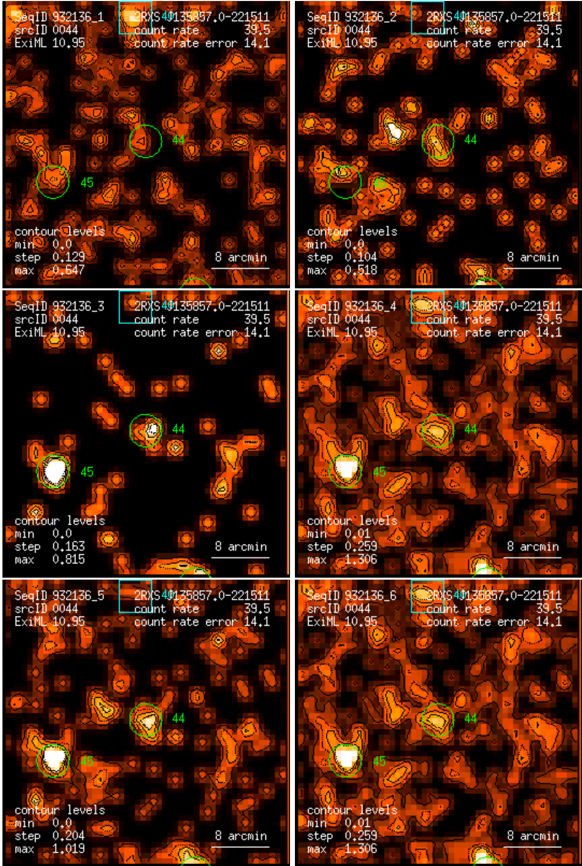
Figure 44: RASS 932136: detection 0044: band rate images, Gaussian filter: (1) PSPC channels 11 – 41, (2) 52 – 90, (3) 91 – 201, (4) 11 – 235, (5) 52 – 201, (6) 11 – 201. Broad band rates in counts/ks. Band rate contour levels in counts/ks/arcmin 2 .
