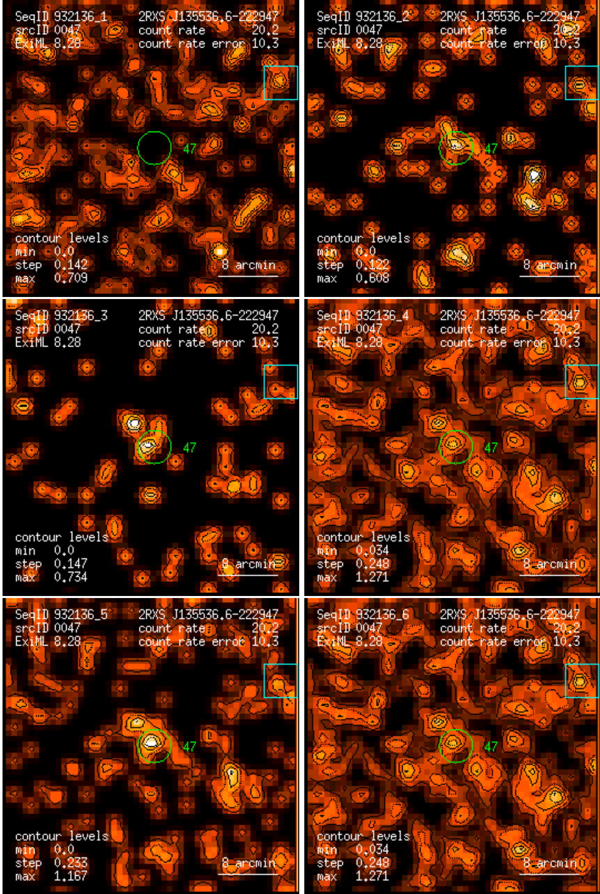
Figure 47: RASS 932136: detection 0047: band rate images, Gaussian filter: (1) PSPC channels 11 – 41, (2) 52 – 90, (3) 91 – 201, (4) 11 – 235, (5) 52 – 201, (6) 11 – 201. Broad band rates in counts/ks. Band rate contour levels in counts/ks/arcmin 2 .
