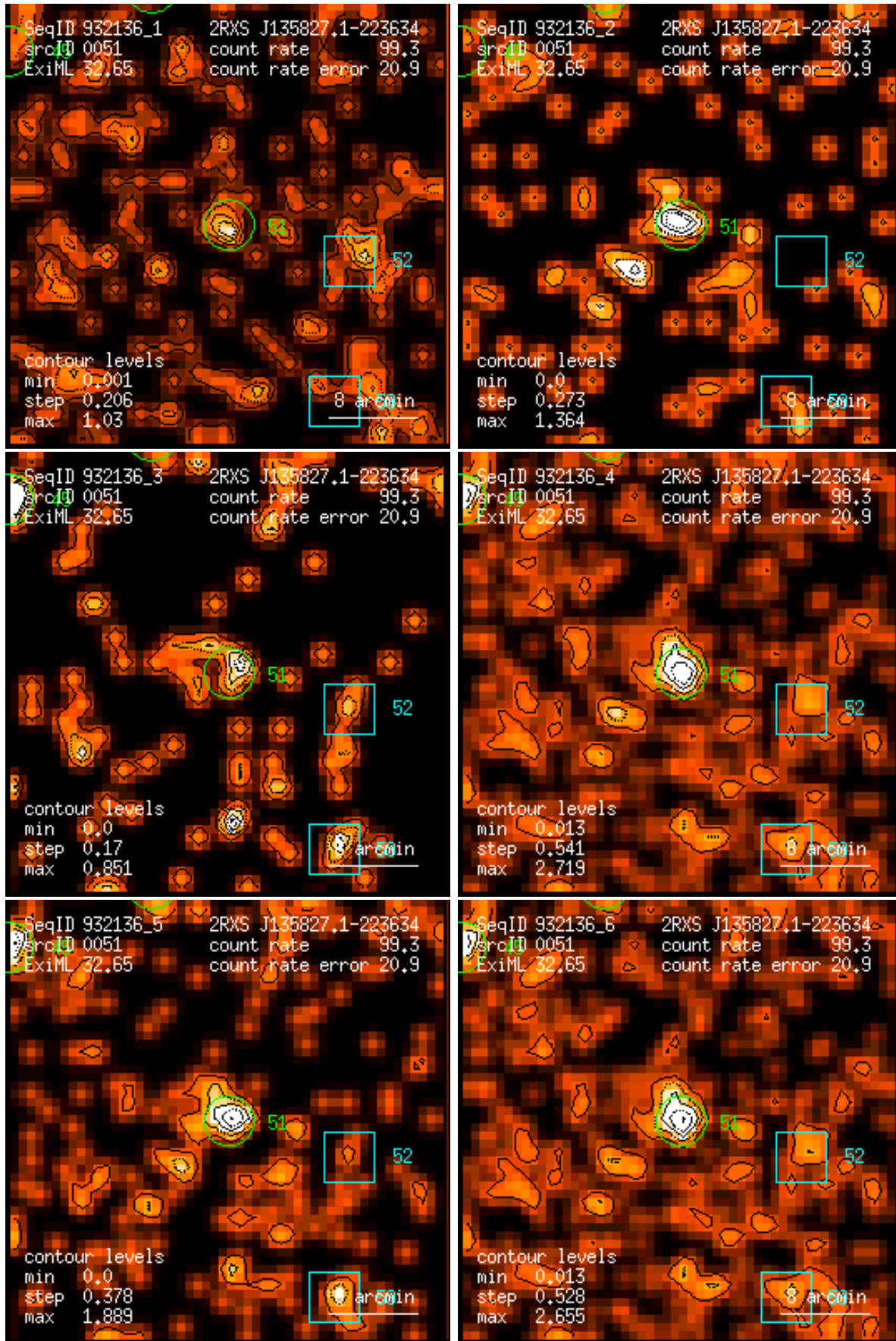
Figure 51: RASS 932136: detection 0051: band rate images, Gaussian filter: (1) PSPC channels 11 – 41, (2) 52 – 90, (3) 91 – 201, (4) 11 – 235, (5) 52 – 201, (6) 11 – 201. Broad band rates in counts/ks. Band rate contour levels in counts/ks/arcmin 2 .
