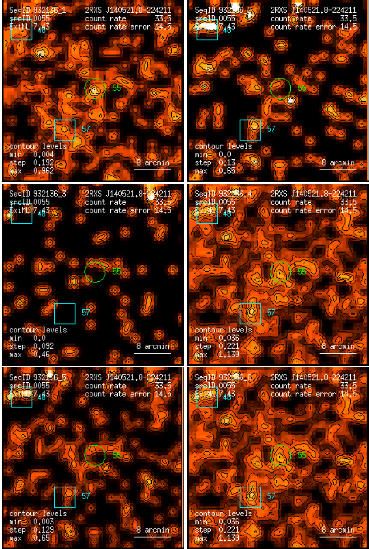
Figure 55: RASS 932136: detection 0055: band rate images, Gaussian filter: (1) PSPC channels 11 – 41, (2) 52 – 90, (3) 91 – 201, (4) 11 – 235, (5) 52 – 201, (6) 11 – 201. Broad band rates in counts/ks. Band rate contour levels in counts/ks/arcmin 2 .
