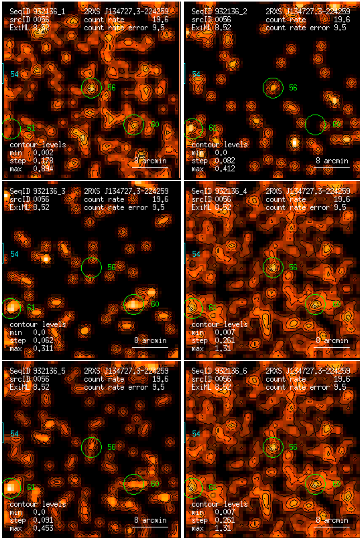
Figure 56: RASS 932136: detection 0056: band rate images, Gaussian filter: (1) PSPC channels 11 – 41, (2) 52 – 90, (3) 91 – 201, (4) 11 – 235, (5) 52 – 201, (6) 11 – 201. Broad band rates in counts/ks. Band rate contour levels in counts/ks/arcmin 2 .
