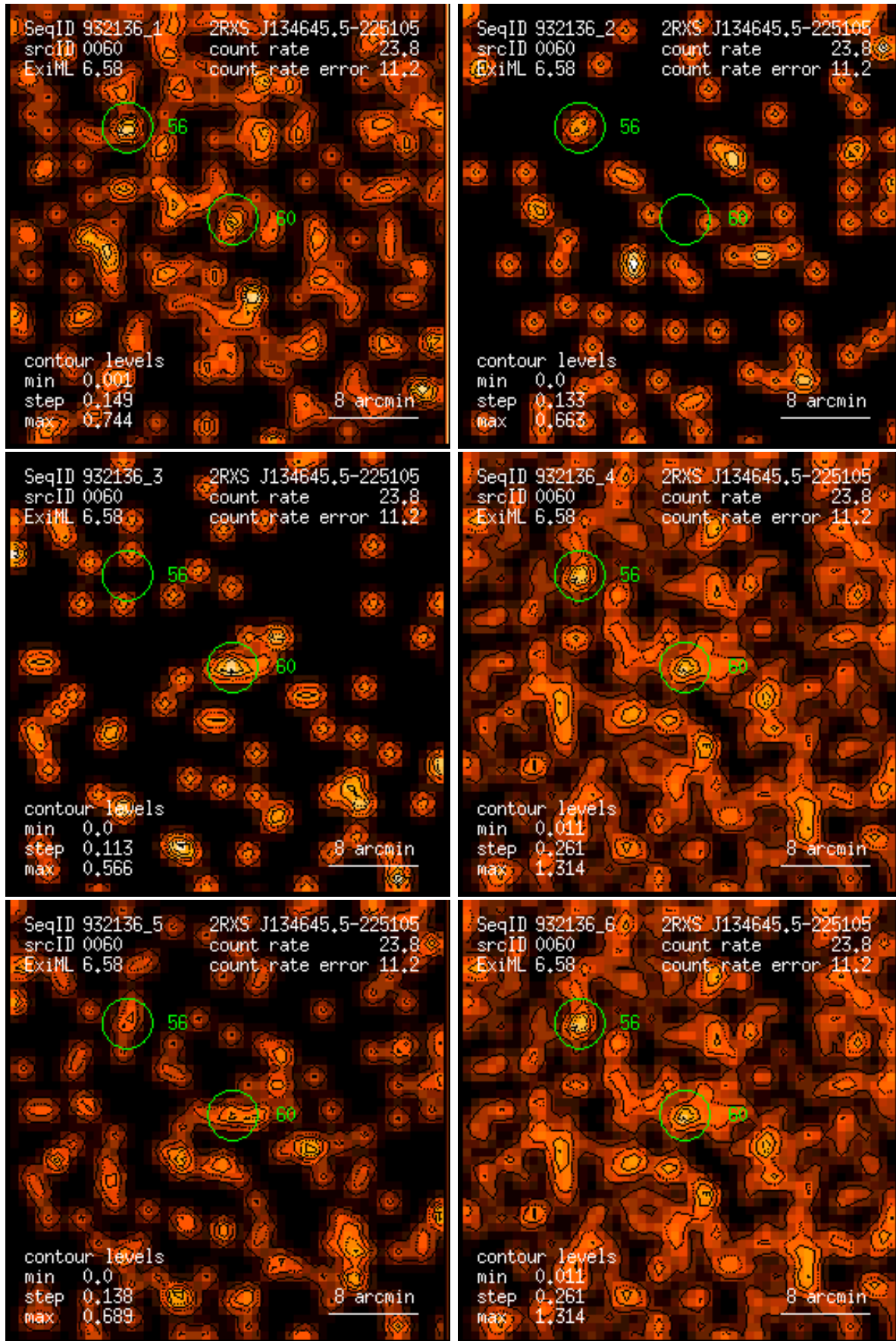
Figure 60: RASS 932136: detection 0060: band rate images, Gaussian filter: (1) PSPC channels 11 – 41, (2) 52 – 90, (3) 91 – 201, (4) 11 – 235, (5) 52 – 201, (6) 11 – 201. Broad band rates in counts/ks. Band rate contour levels in counts/ks/arcmin 2 .
