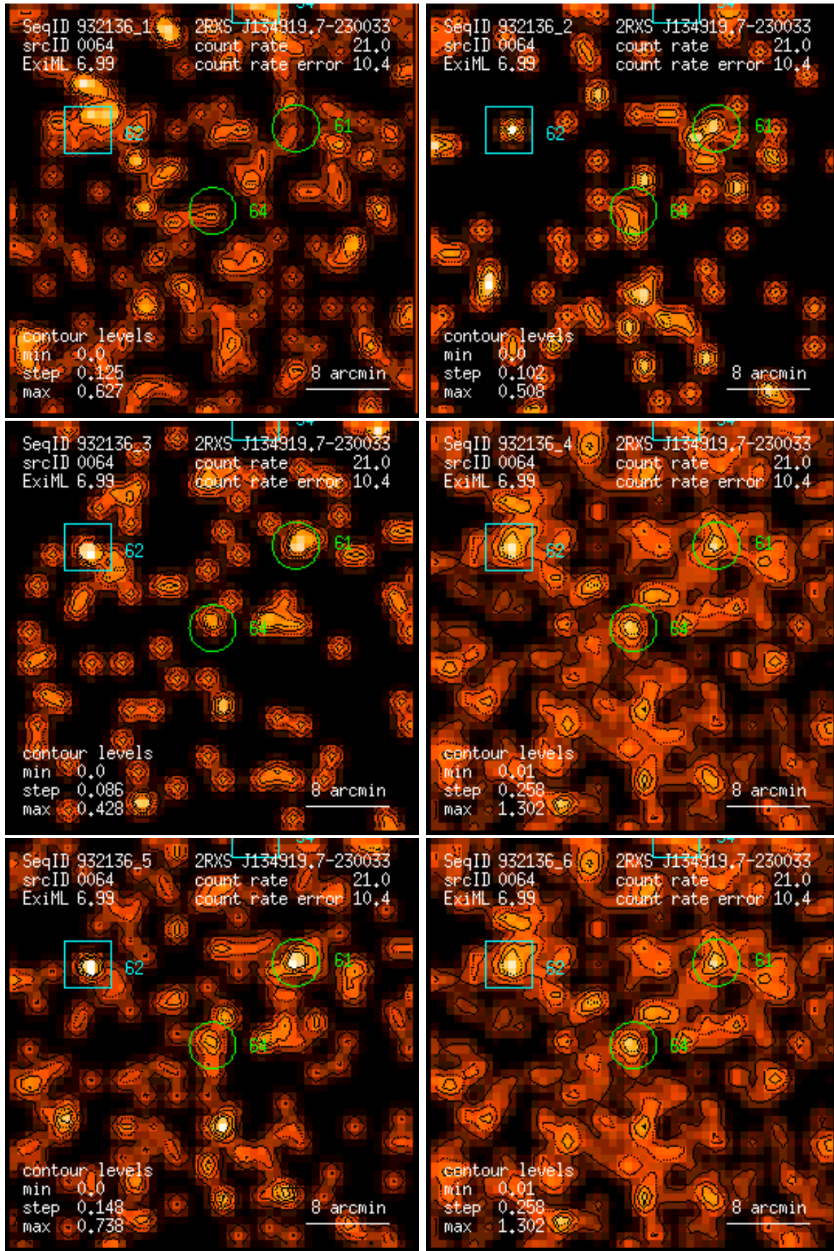
Figure 64: RASS 932136: detection 0064: band rate images, Gaussian filter: (1) PSPC channels 11 – 41, (2) 52 – 90, (3) 91 – 201, (4) 11 – 235, (5) 52 – 201, (6) 11 – 201. Broad band rates in counts/ks. Band rate contour levels in counts/ks/arcmin 2 .
