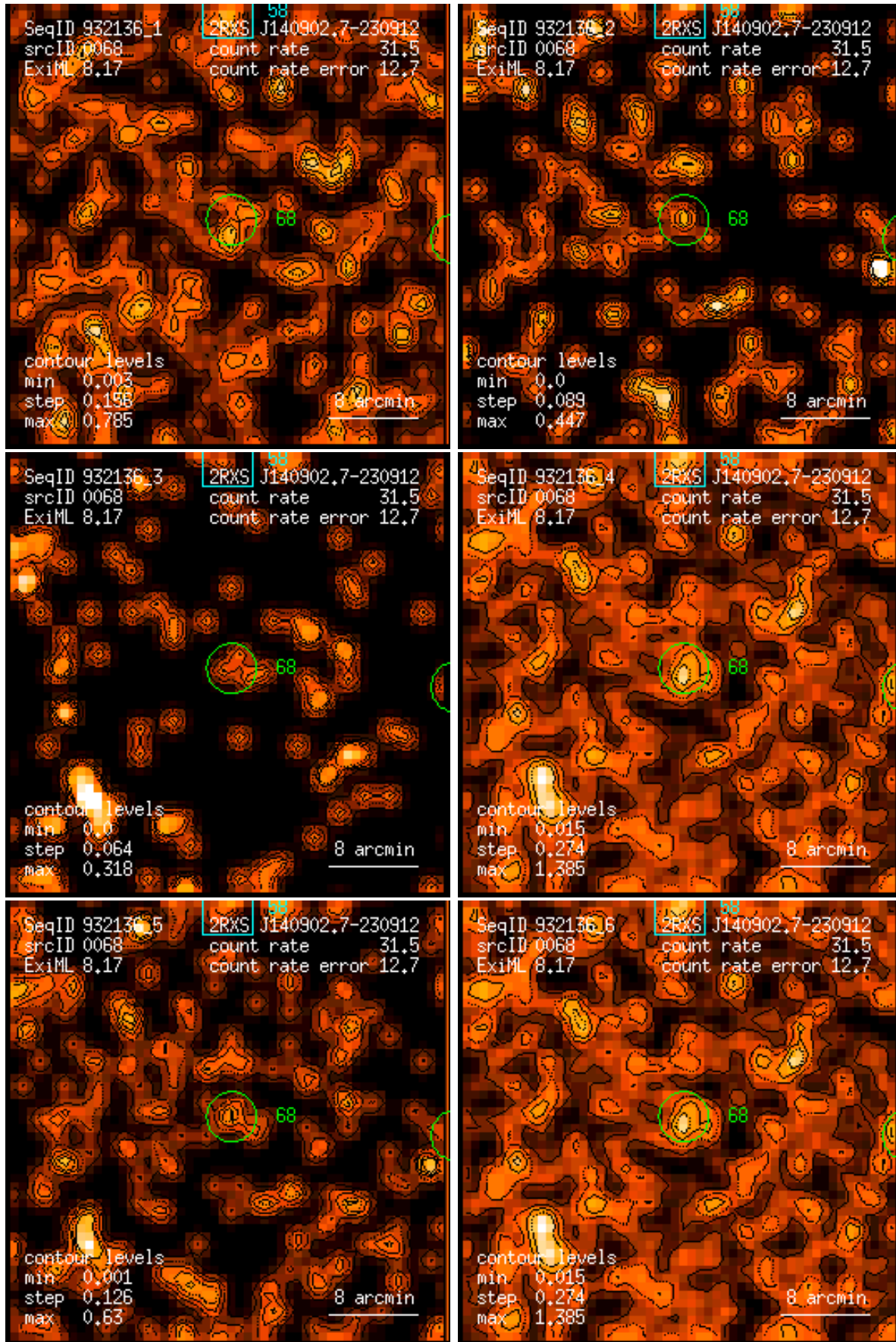
Figure 68: RASS 932136: detection 0068: band rate images, Gaussian filter: (1) PSPC channels 11 – 41, (2) 52 – 90, (3) 91 – 201, (4) 11 – 235, (5) 52 – 201, (6) 11 – 201. Broad band rates in counts/ks. Band rate contour levels in counts/ks/arcmin 2 .
