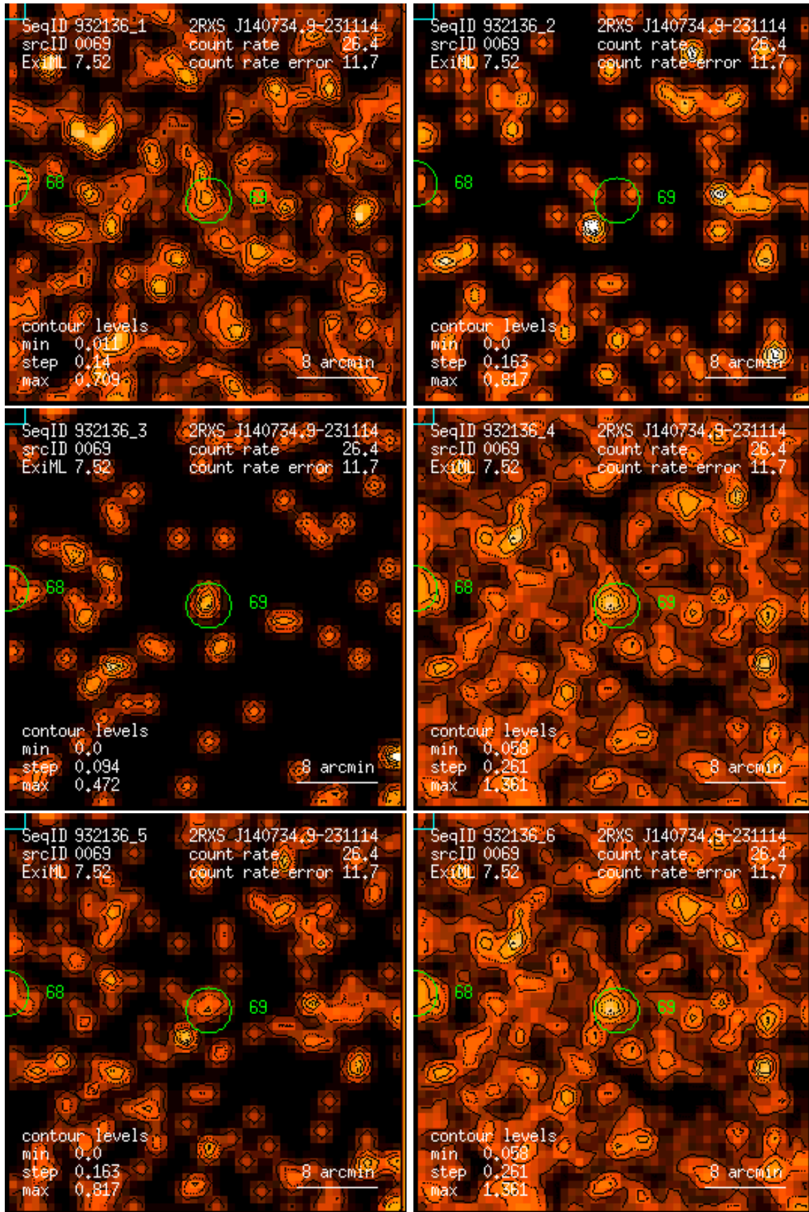
Figure 69: RASS 932136: detection 0069: band rate images, Gaussian filter: (1) PSPC channels 11 – 41, (2) 52 – 90, (3) 91 – 201, (4) 11 – 235, (5) 52 – 201, (6) 11 – 201. Broad band rates in counts/ks. Band rate contour levels in counts/ks/arcmin 2 .
