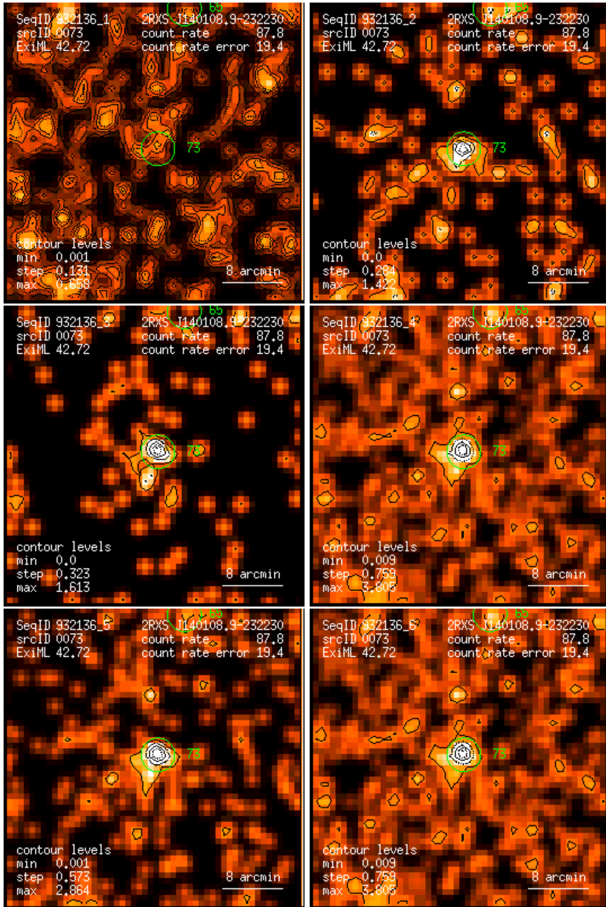
Figure 73: RASS 932136: detection 0073: band rate images, Gaussian filter: (1) PSPC channels 11 – 41, (2) 52 – 90, (3) 91 – 201, (4) 11 – 235, (5) 52 – 201, (6) 11 – 201. Broad band rates in counts/ks. Band rate contour levels in counts/ks/arcmin 2 .
