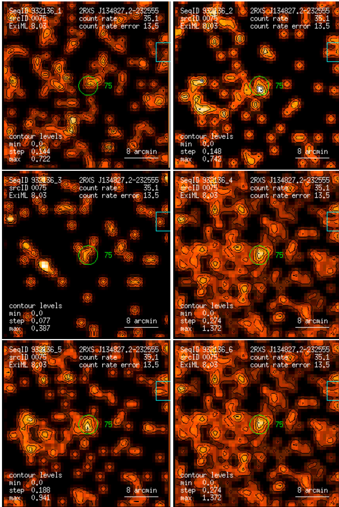
Figure 75: RASS 932136: detection 0075: band rate images, Gaussian filter: (1) PSPC channels 11 – 41, (2) 52 – 90, (3) 91 – 201, (4) 11 – 235, (5) 52 – 201, (6) 11 – 201. Broad band rates in counts/ks. Band rate contour levels in counts/ks/arcmin 2 .
