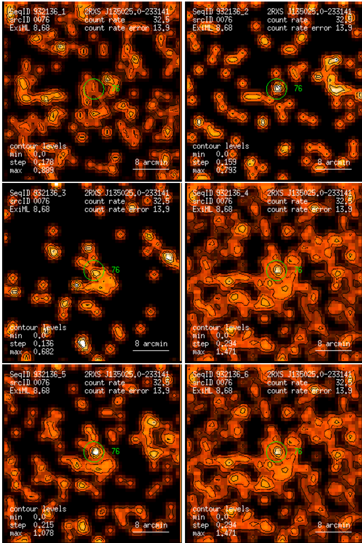
Figure 76: RASS 932136: detection 0076: band rate images, Gaussian filter: (1) PSPC channels 11 – 41, (2) 52 – 90, (3) 91 – 201, (4) 11 – 235, (5) 52 – 201, (6) 11 – 201. Broad band rates in counts/ks. Band rate contour levels in counts/ks/arcmin 2 .
