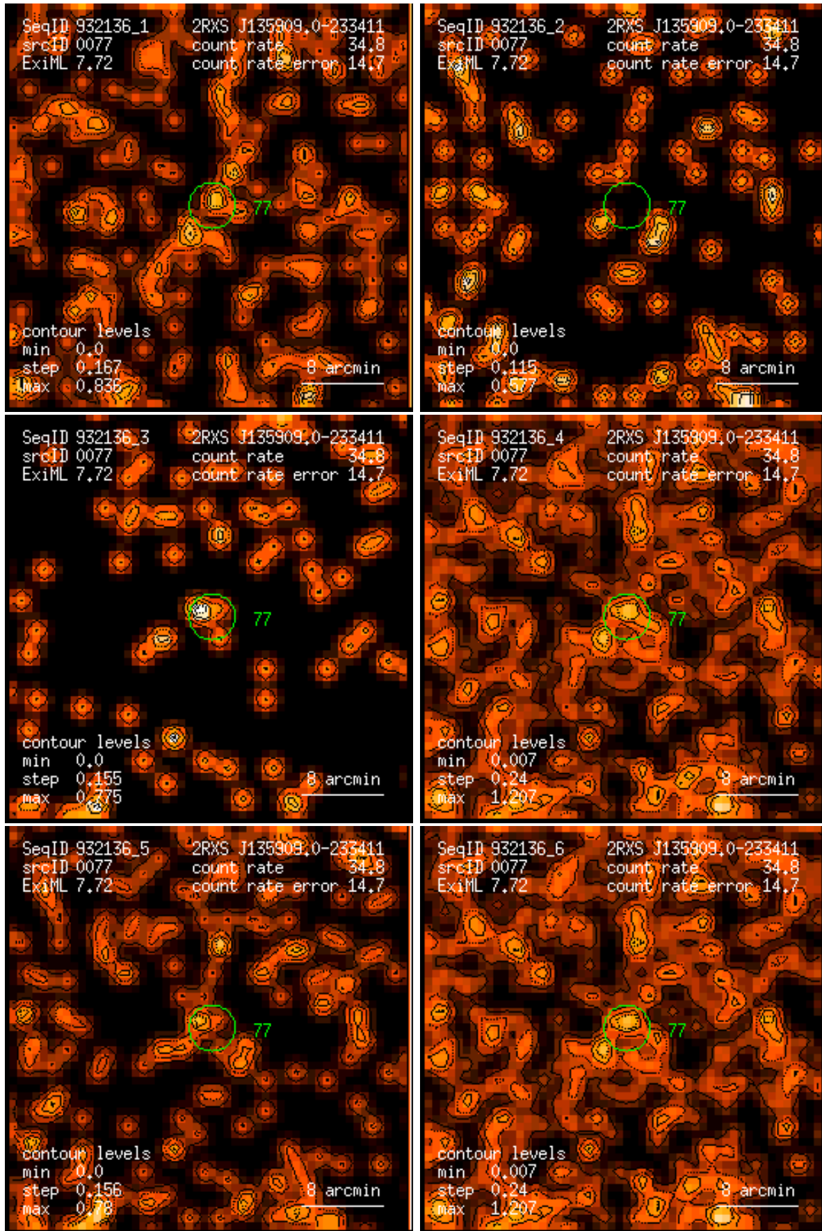
Figure 77: RASS 932136: detection 0077: band rate images, Gaussian filter: (1) PSPC channels 11 – 41, (2) 52 – 90, (3) 91 – 201, (4) 11 – 235, (5) 52 – 201, (6) 11 – 201. Broad band rates in counts/ks. Band rate contour levels in counts/ks/arcmin 2 .
