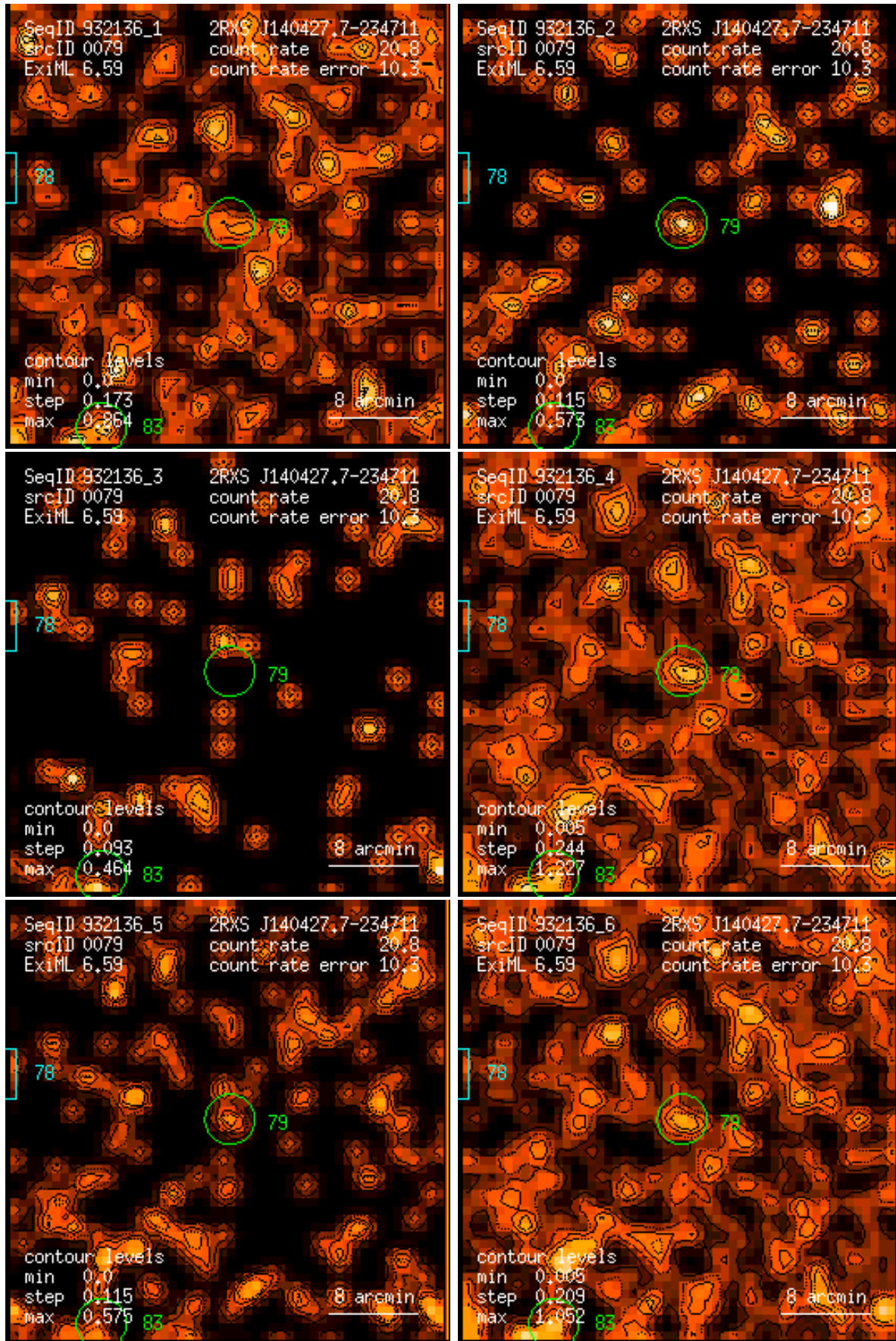
Figure 79: RASS 932136: detection 0079: band rate images, Gaussian filter: (1) PSPC channels 11 – 41, (2) 52 – 90, (3) 91 – 201, (4) 11 – 235, (5) 52 – 201, (6) 11 – 201. Broad band rates in counts/ks. Band rate contour levels in counts/ks/arcmin 2 .
